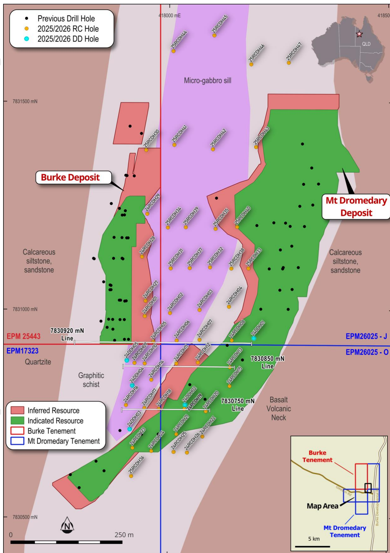
Figure 1: Completed drill holes within Burke and Mt Dromedary Deposits and Cross-Section Lines - current Indicated and Inferred Mineral Resources Plan View and Geology
