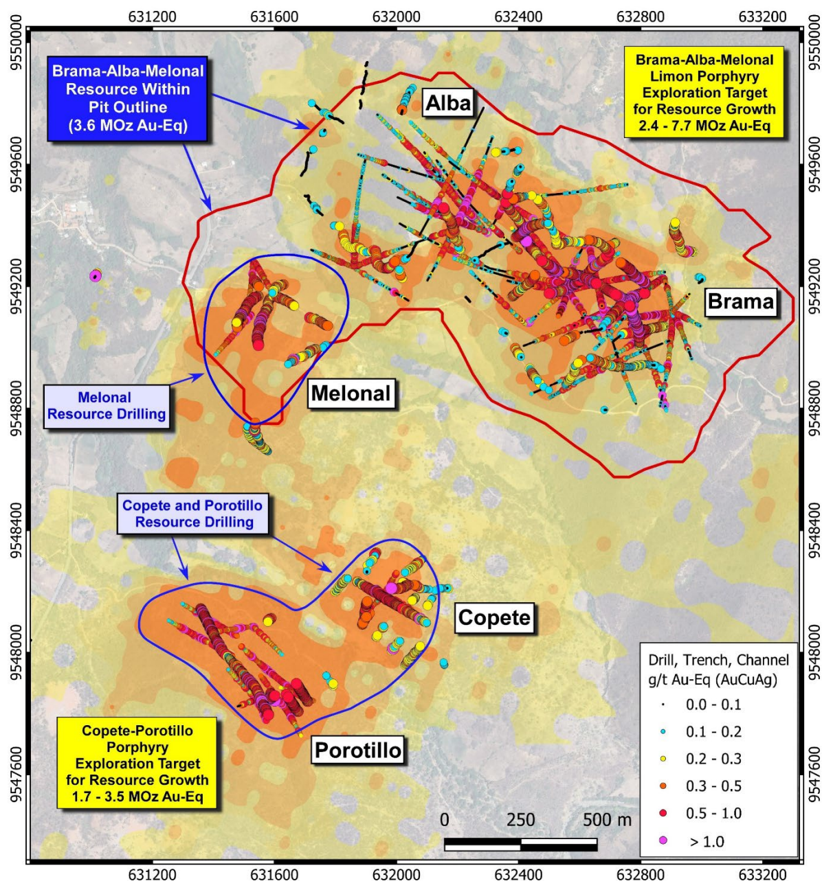
Figure 3: The cluster of five porphyry gold-copper systems in the Bramaderos concessions (Brama, Alba, Melonal, Copete and Porotillo), and showing the area where resource drilling in the current drill program has been underway at Porotillo, Copete and Melonal to grow the Bramaderos Mineral Resource. Background colour shading is gold in soils.
