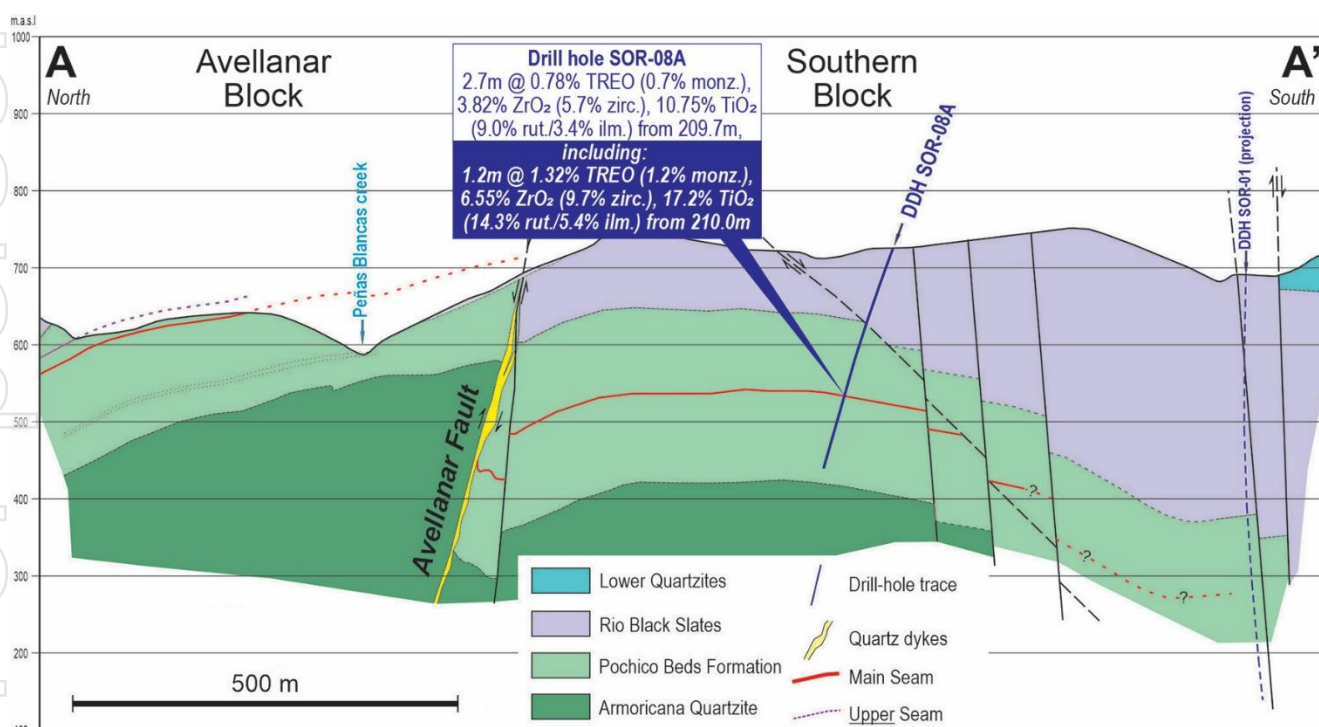
Figure 4 – SOR-08A cross-section.
