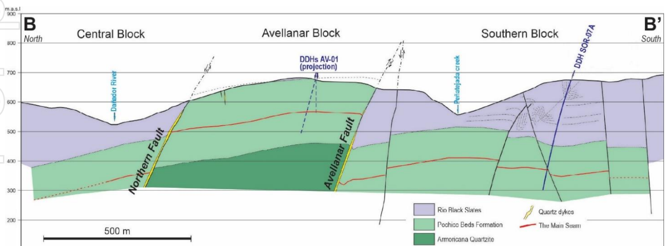
Figure 6 – SOR-07A cross-section
