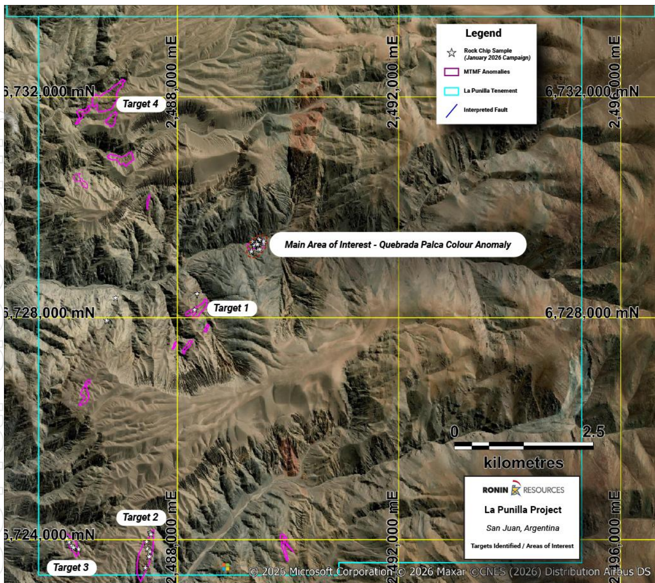
Figure 2: La Punilla Project – Main Area of Interest (Quebrada Palca Colour Anomaly) showing targets identified, MTMF anomalies and all rock chip samples from the January 2026 campaign. Map indicates the new work which was undertaken in January 2026; new sample locations are shown with star symbols, MTMF anomalies by magenta-coloured polygons, and purple lines represent interpreted faults.
