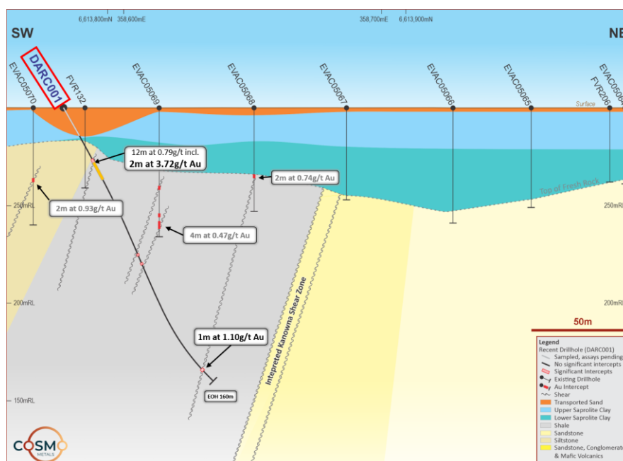
Figure 3. Cross Section – Don Alvaro DARC001
