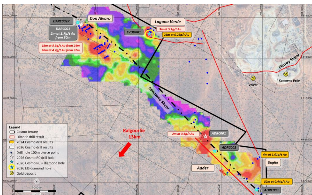
Figure 2. Kanowna Gold Project, CMO drilling on aerial photo showing all previous drilling below 100m vertical
