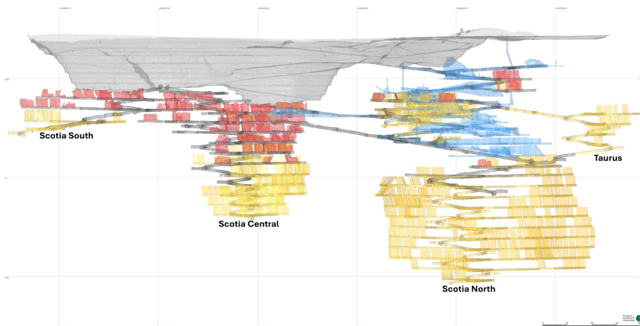
Figure: Scotia Underground Mine showing current development, planned development and stopes.
