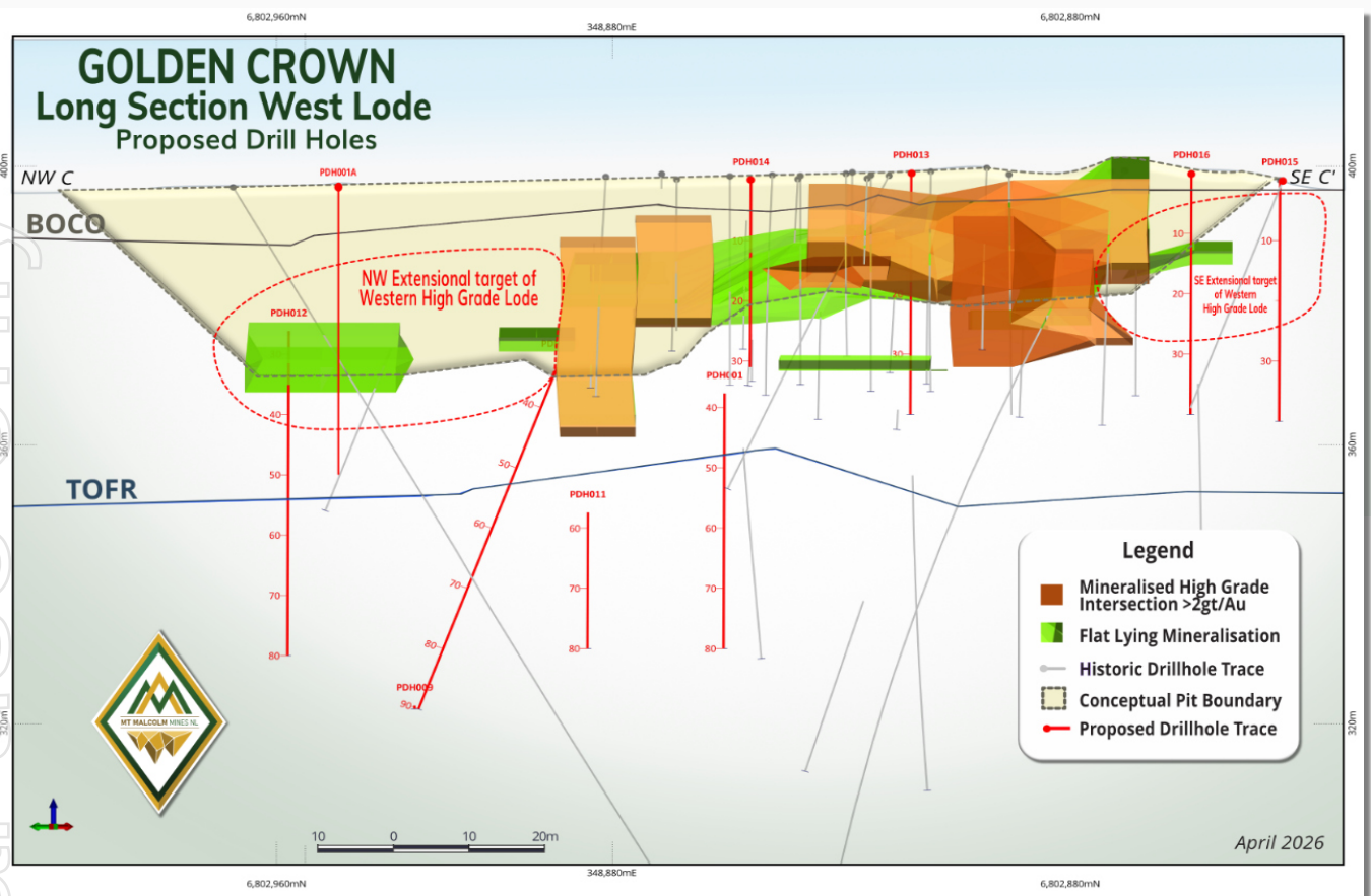
Figure 3. Golden Crown long section — planned holes on Western Lode, high-grade shoot. (refer ASX announcement 16 July 2026).
