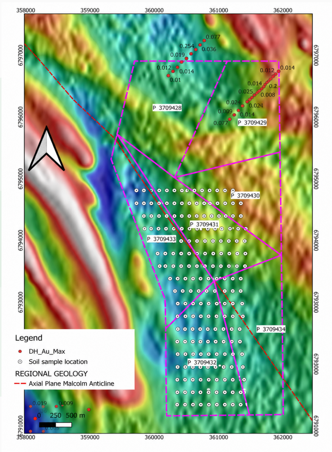
Figure 8B. Wool Shed regional pXRF soil program sample locations over TMI.
