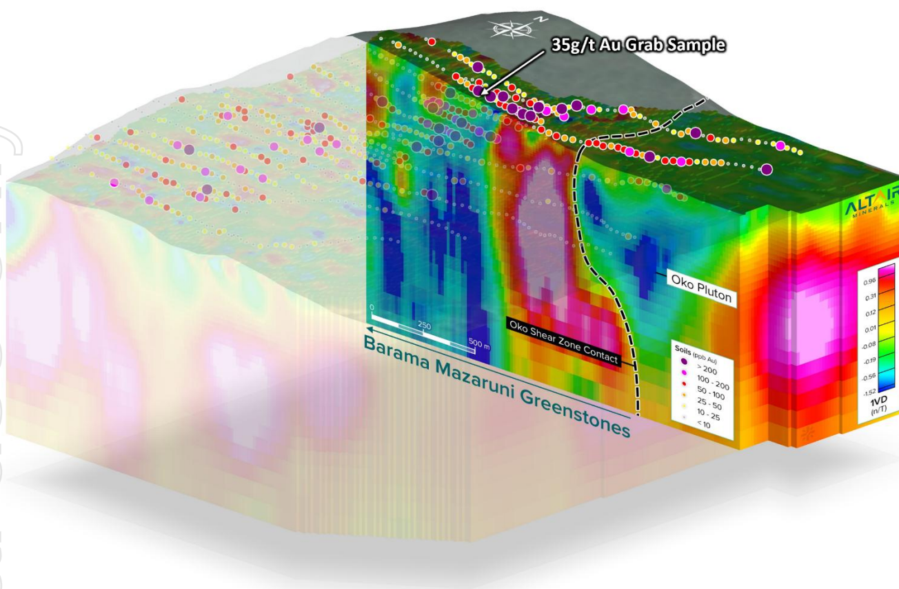
Figure 9: 3D view of magnetic inversion at SOKO, cut at 695200N (WGS84, UTM Zone 21N), with soil samples to date overlaid. 24,33
