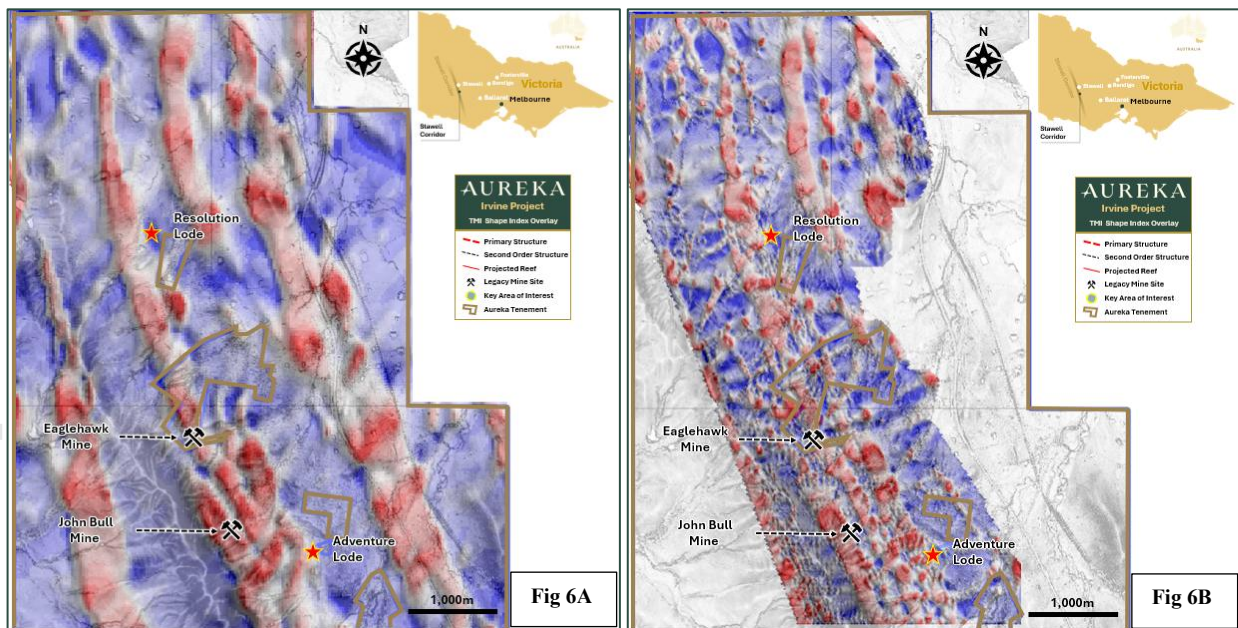
Figure 6 A&B. Side by side comparison between the reprocessed legacy TMI shape index magnetics data (Fig A) with the newly acquired drone magnetics data (Fig B). The tighter 50m-spaced drone magnetics provides enhanced local-scale resolution enabling identification of contrasting magnetic responses and possible emerging second order structures that provide further local scale targeting opportunities with potential to deliver new mineral discoveries at Irvine
