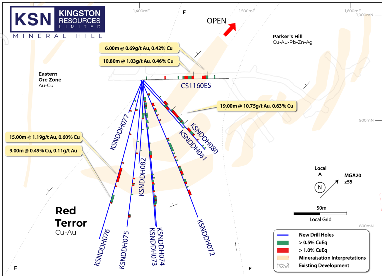
Figure 6: Red Terror drilling results, indicating potential extension of high-grade gold and copper to the south.
