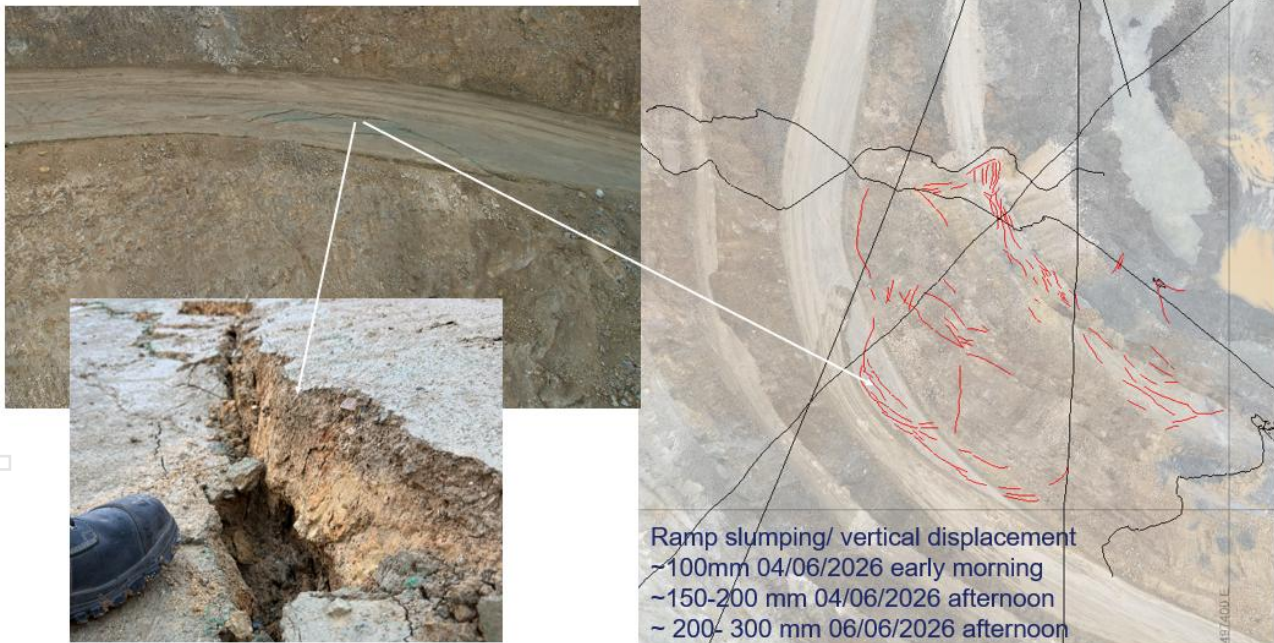
Figure 1: Pearse South Open Pit tension cracks and slumping in the ramp on the southern wall.
