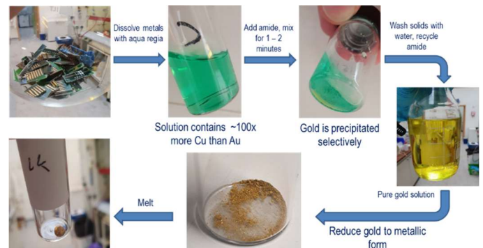
Figure 4 – Gold Extraction using Diamide Ligand Technology
