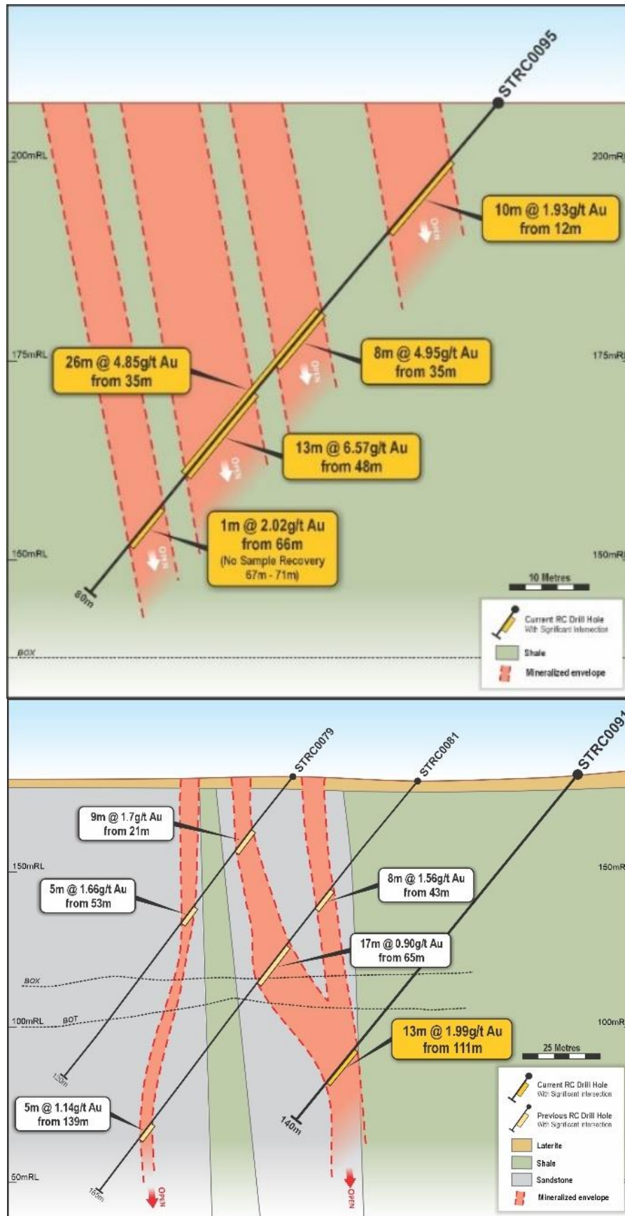
Figure 4 – Satama Cross Sections STRC0095 and STRC009. See Figure 3 for Section location. (refer TCG ASX announcement dated 10 October 2023).
