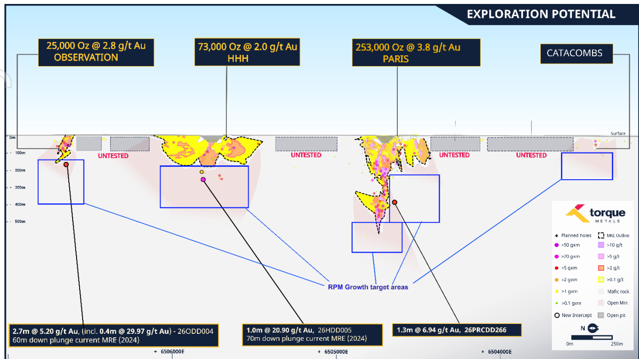
Figure 6: Long Section of the Paris Gold Project, highlighting scale across multiple high-grade deposits
