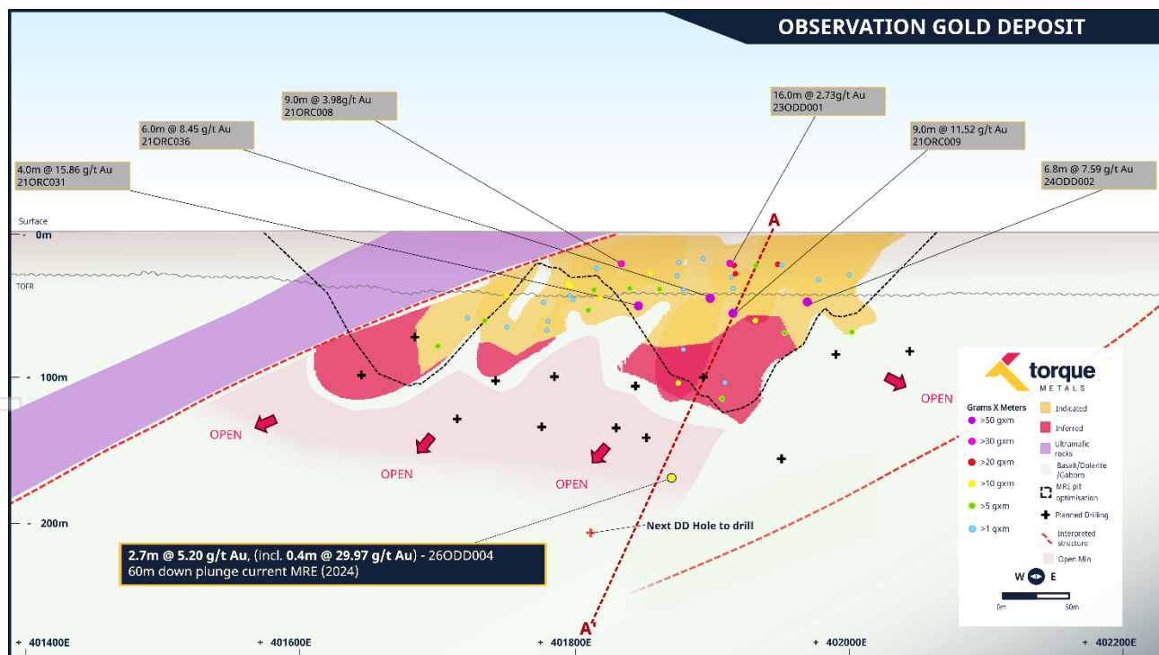
Figure 2: Long section of Observation Gold Deposit showing the current MRE outline and the recent drilling intercept
