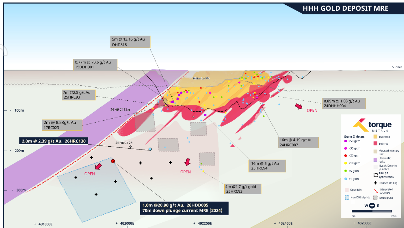
Figure 4: HHH long section showing the new intercept points below the current MRE outline, and the new DHEM plate projecting mineralisation down-plunge.
