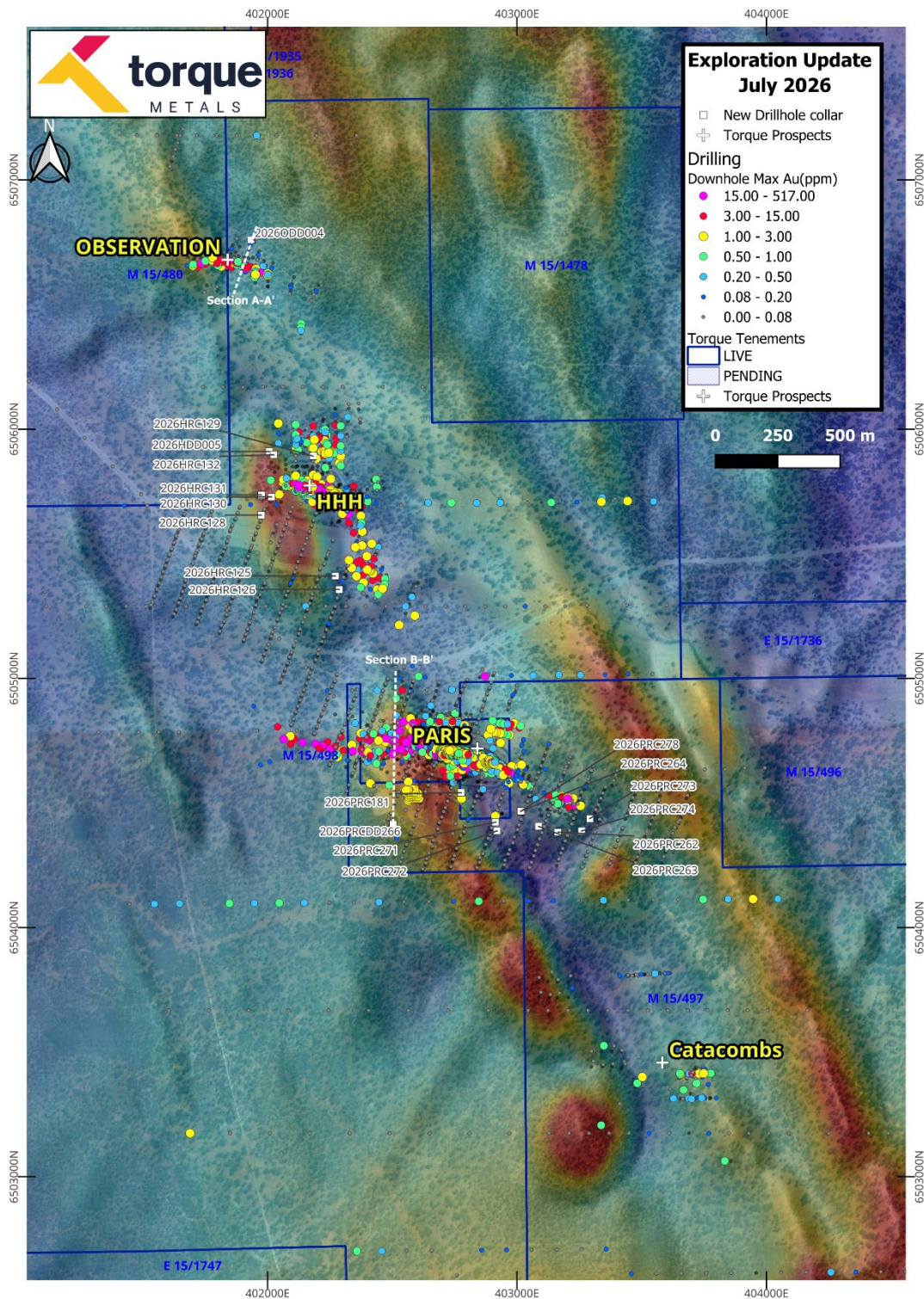
Figure 1: Plan view of the Paris Corridor and new drill-hole locations for this announcement with the regional magnetics
