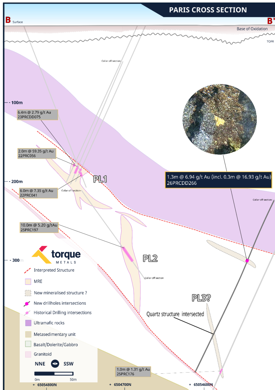
Figure 5: Cross-section through 26PRCDD266 showing a new result and interpreted structures intersected.
