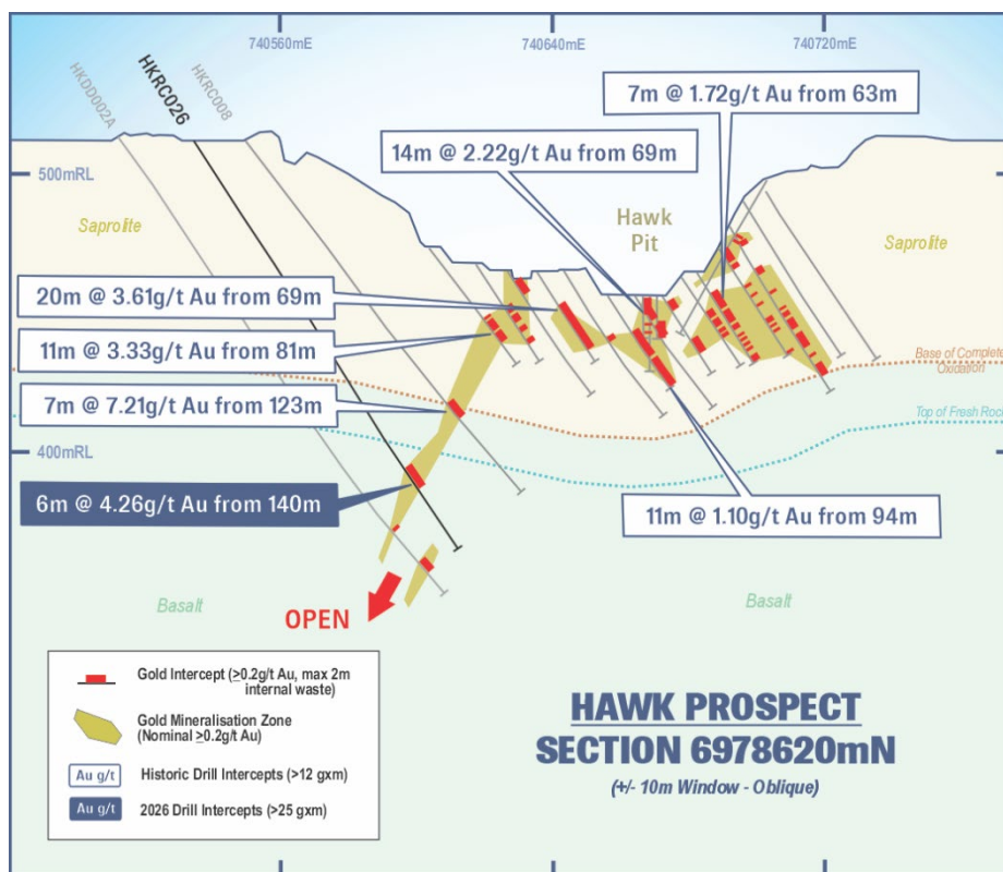
Figure 5: Hawk cross section showing interpreted mineralised zones, 2026 RC intercepts ( >25\text{ GxM} ) and historic intercepts ( >12\text{ GxM} ) labelled.
