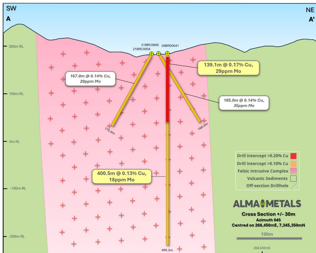
Figure 3. Cross-Section for hole 26BRD0041. Location of section depicted as dashed line AA' on Figure 1.
