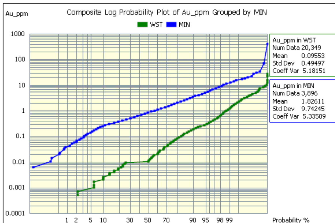
Figure 5: Au Log Probability Plot by Domain
