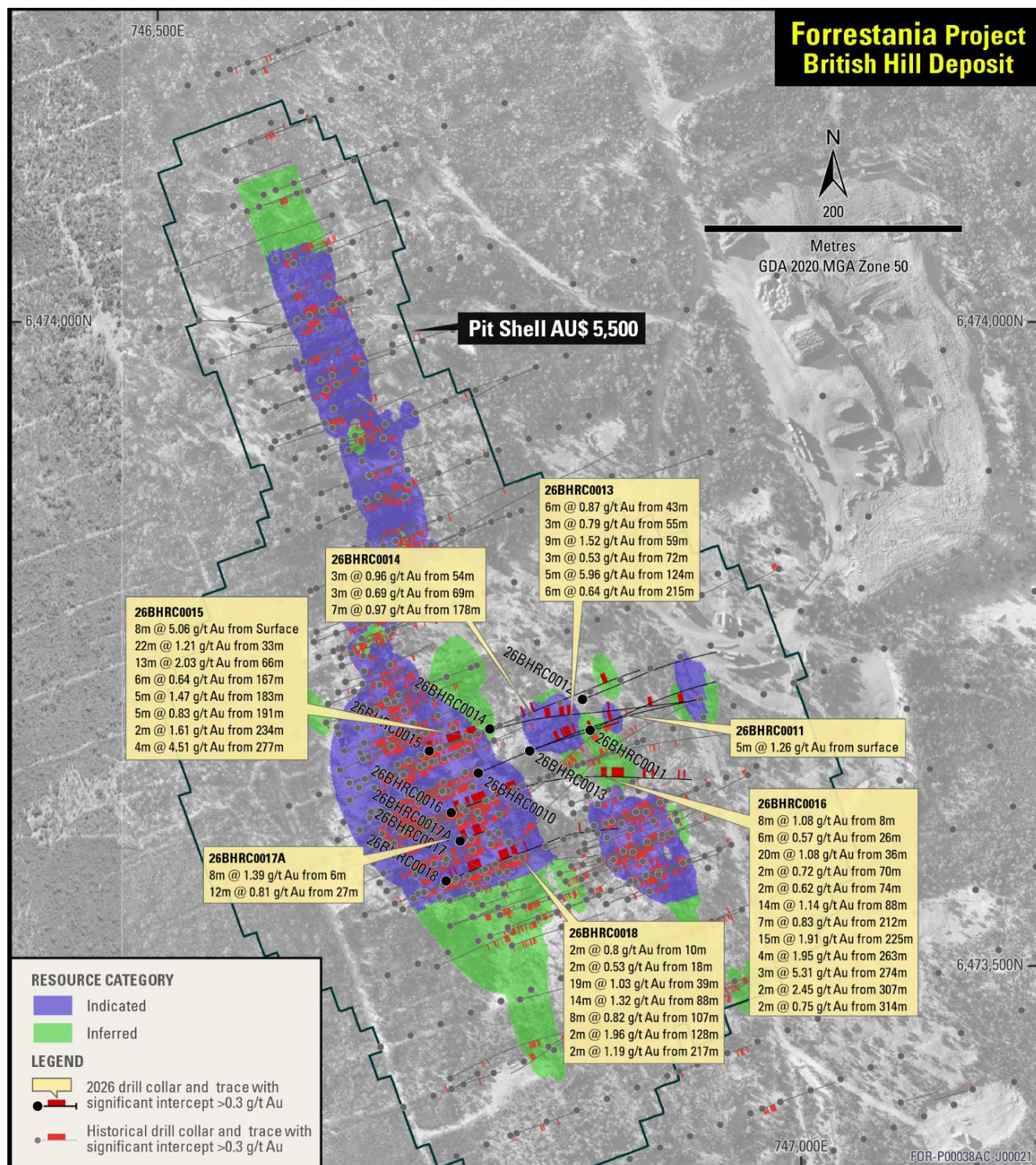
Figure 4: British Hill Deposit – Resource Category
