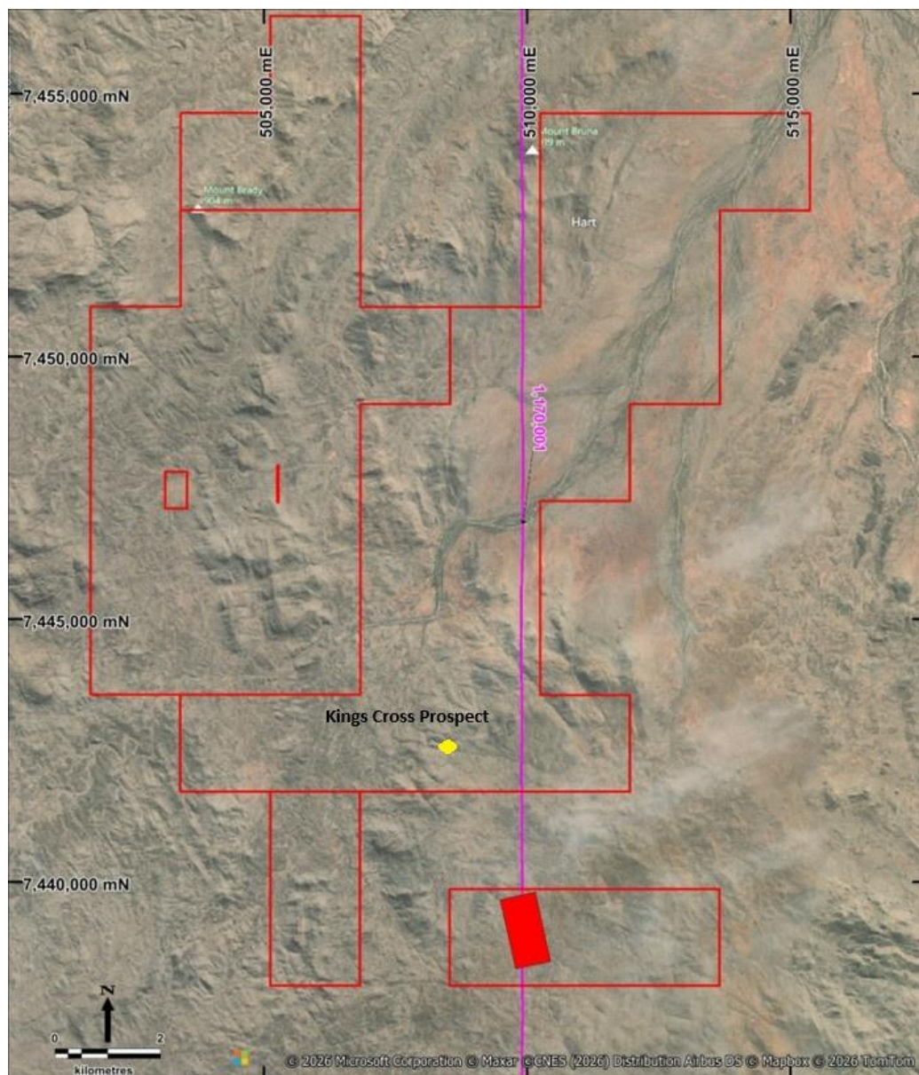
Figure 2: Aerial view of the location of the modelled red plate relative to adjacent NFM Harts Range tenure, shown over AusAEM Line 1170001 in purple (source SGC, 2026 modelling) 1
