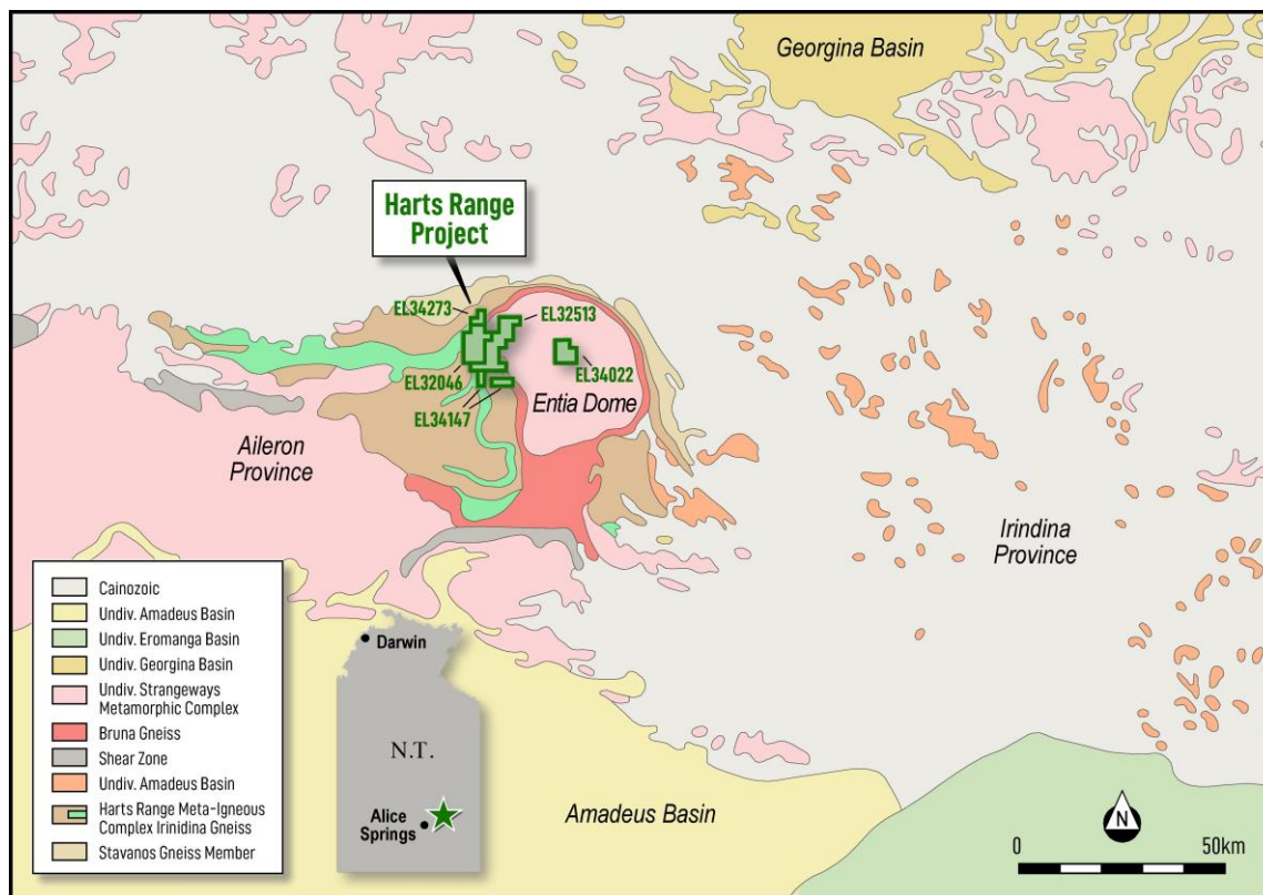
Figure 1: Regional geological setting and NFM tenement position
