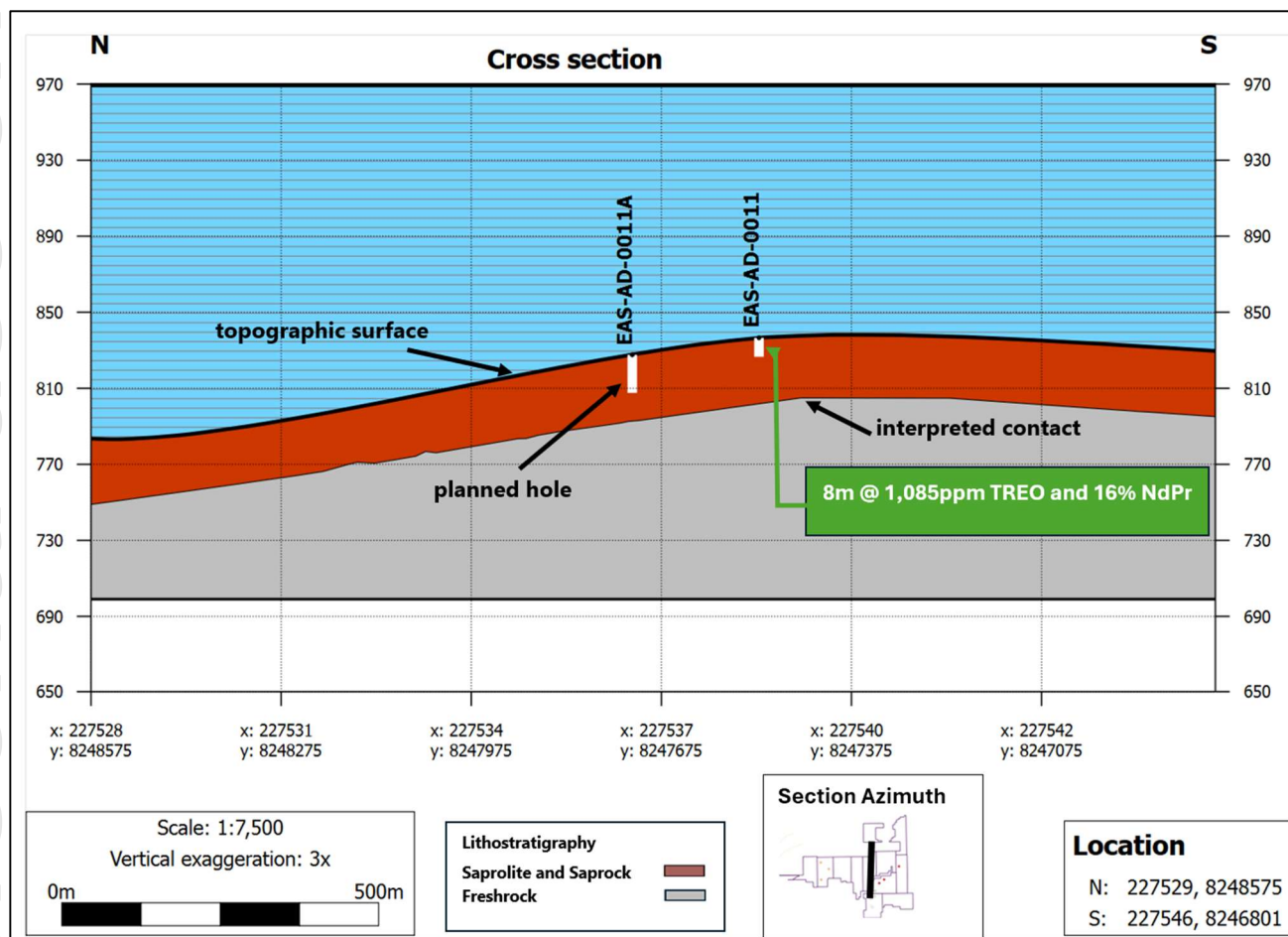
Figure 5: Schematic interpreted cross section through EAS-AD-0011 in East Salinas (Planned hole may vary in position and depth based on the access and auger drilling capability)
