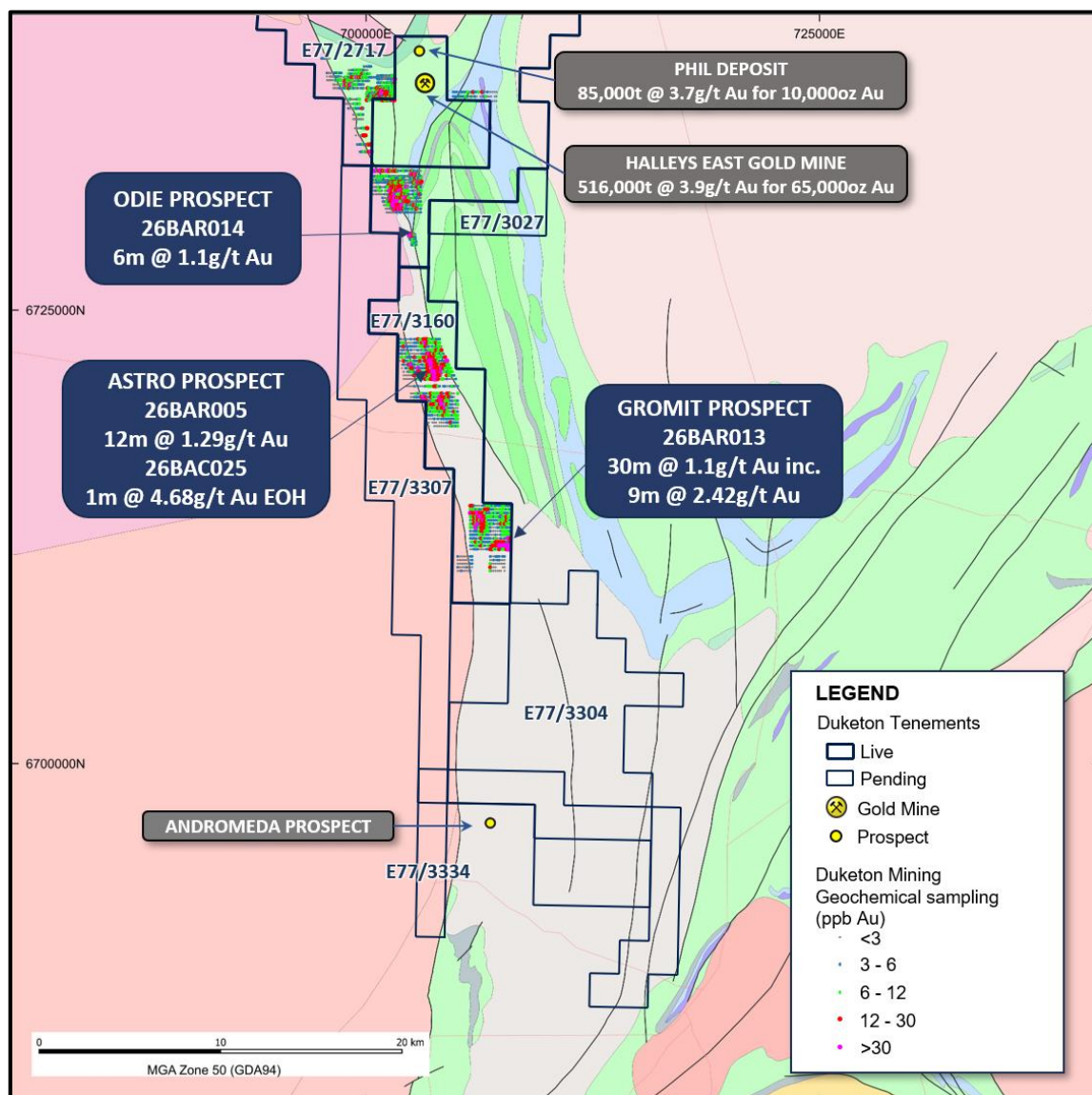
Figure 1: UFF soil geochemistry, drillhole locations and Prospects over Interpreted Bedrock Geology (GSWA), Barlee Project
