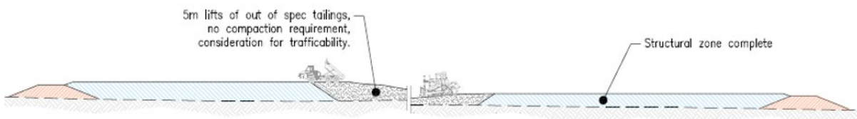
Figure 10.5: TSF Non-Structural Zone First Lift
