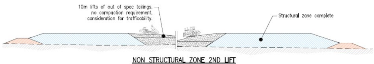
Figure 10.6: TSF Subsequent Lifts
