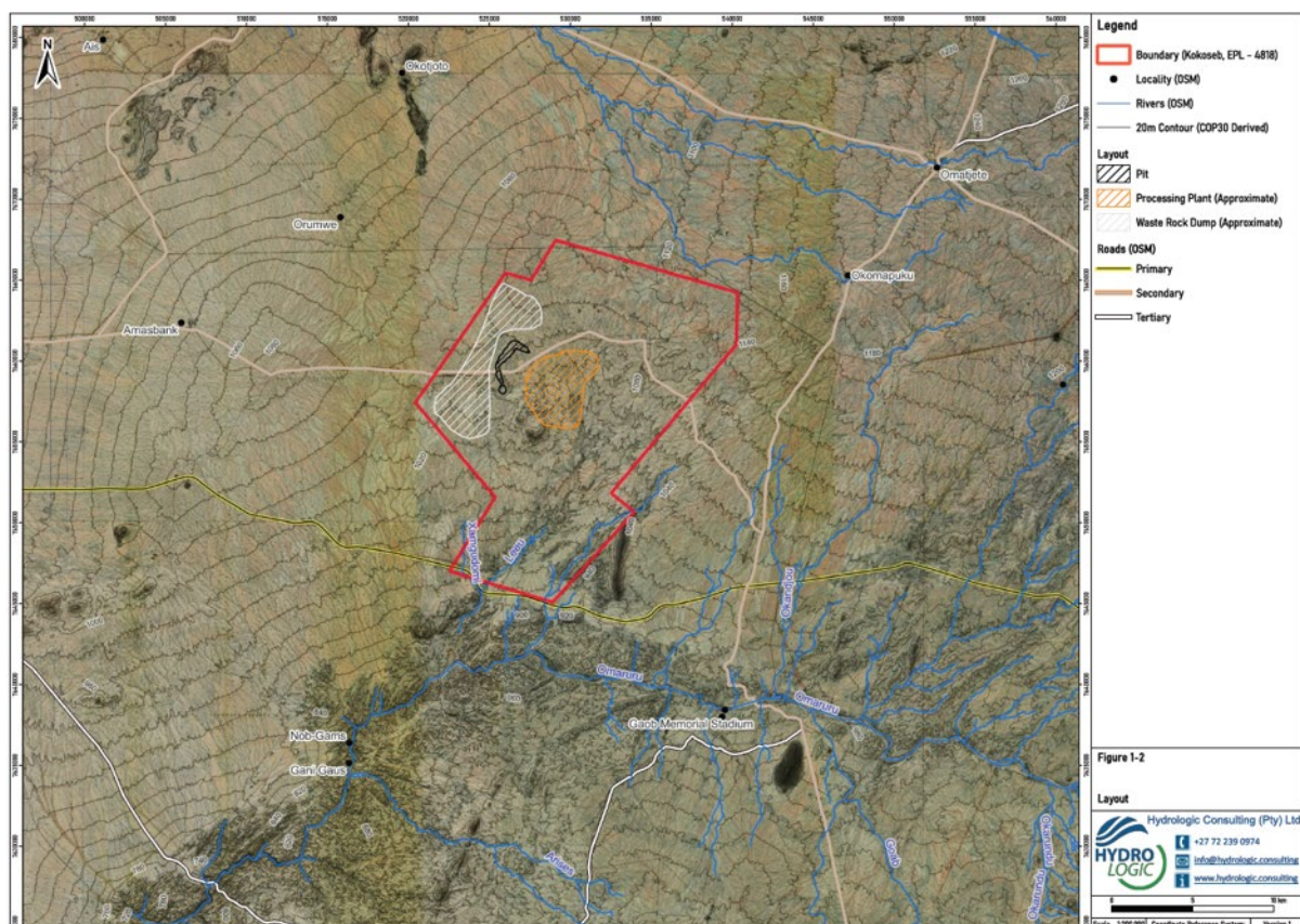
Figure 6.4: Regional Site Layout
