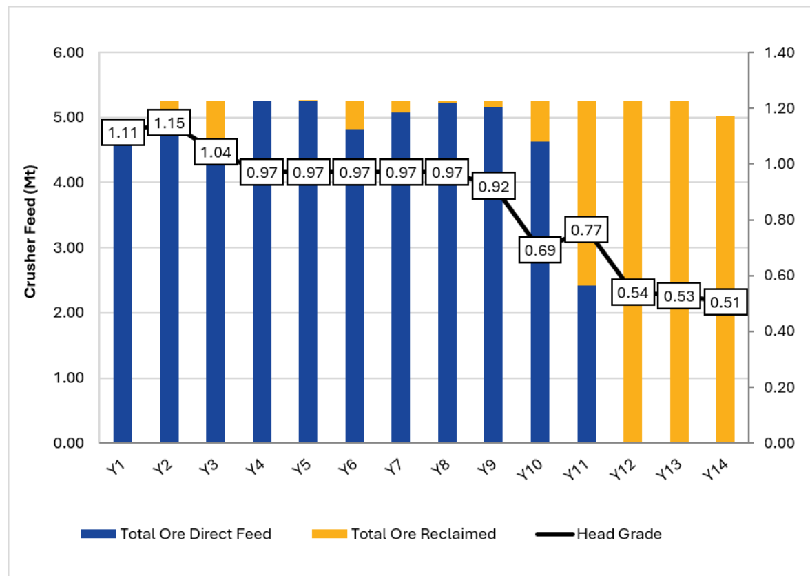
Figure 8.23: Annual Mill Feed and Grade
