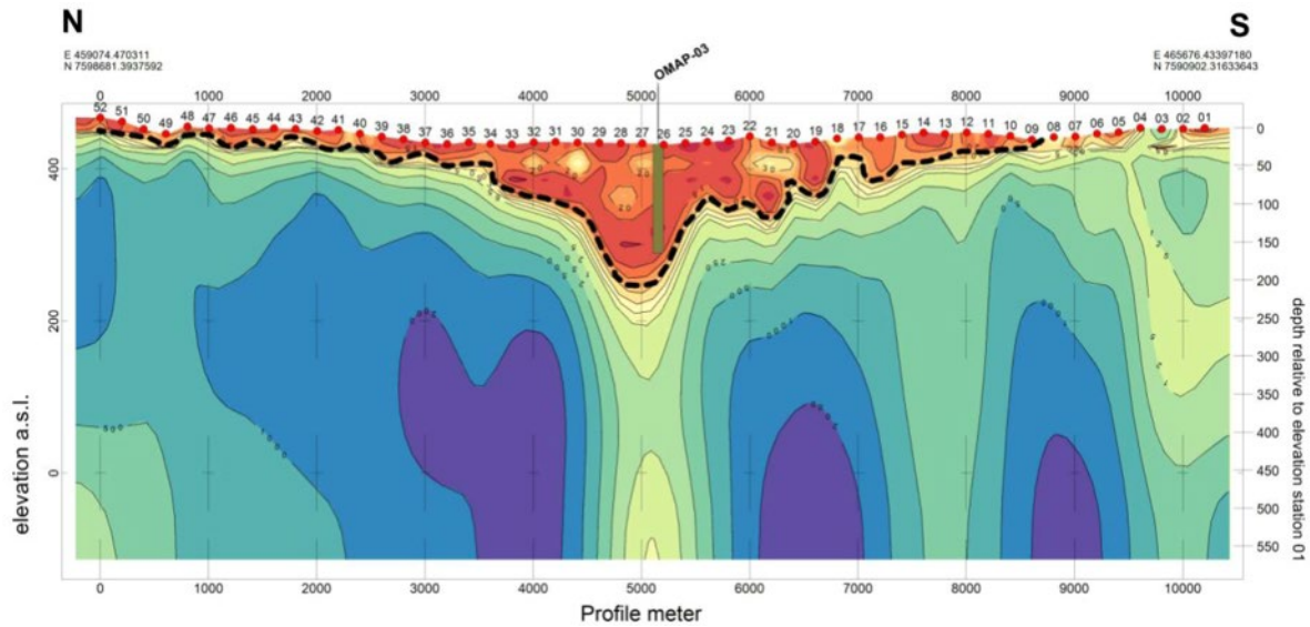
Figure 11.8: NSAMT Profile 4
