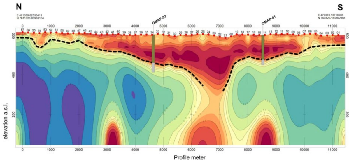
Figure 11.9: NSAMT Profile 6
