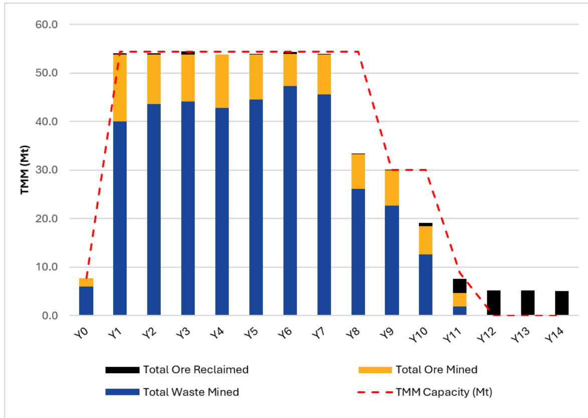
Figure 8.21: Annual Total Material Movement
