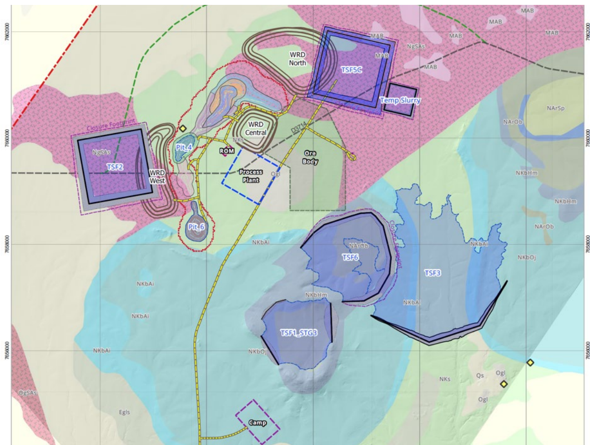
Figure 10.1: Initial Locations Considered for the TSF in the MCAA Process
