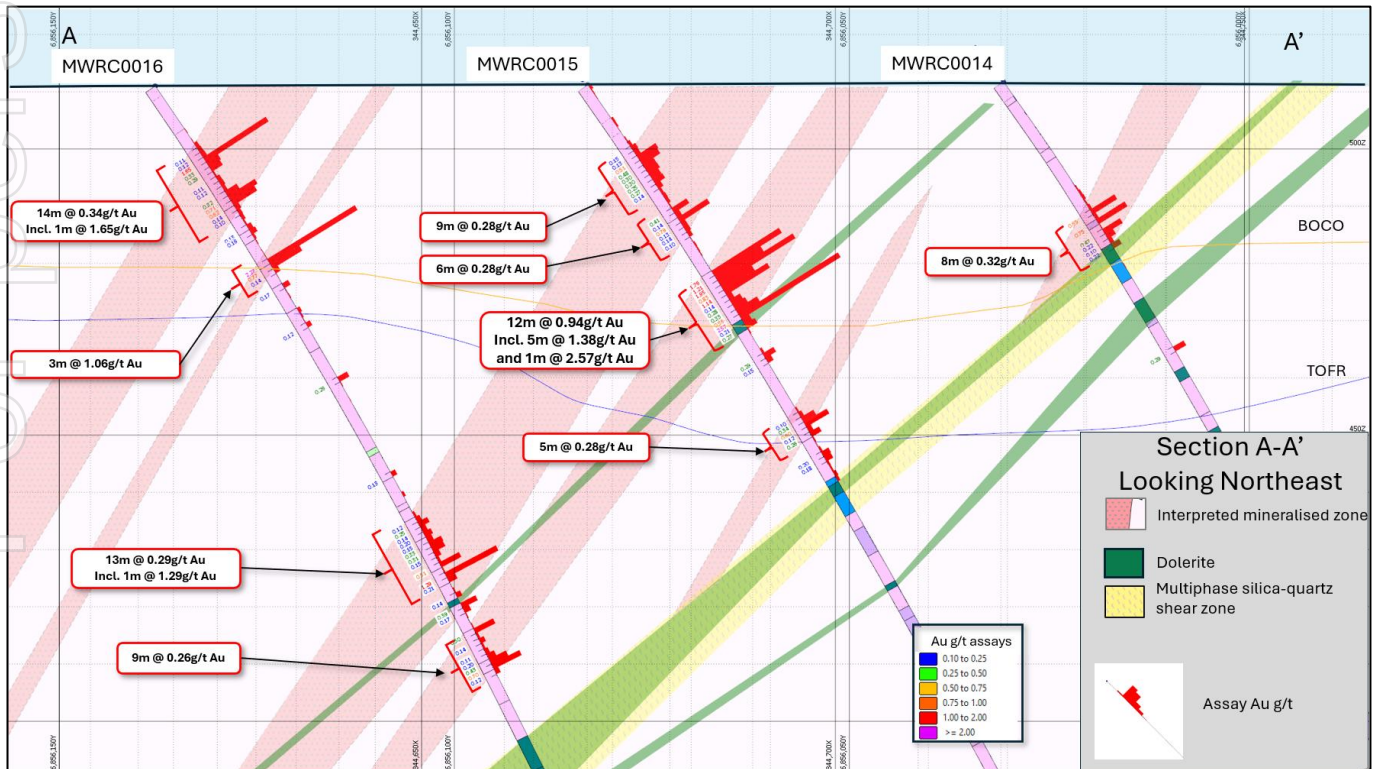
Figure 4 Cross Section A-A' showing assays >0.1g/t Au and interpreted mineralised zones.
