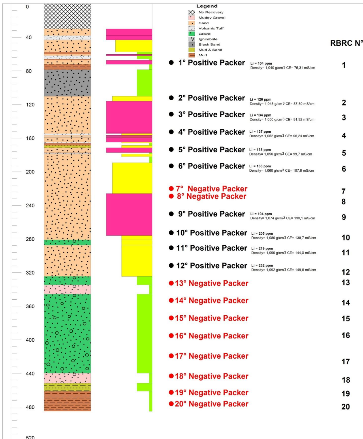
Figure 4. Summary of the lithological column with packer test site annotation focused on SG increasing.
