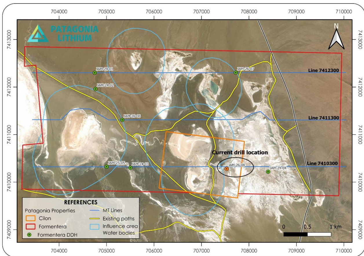
Figure 1. Map of location of well JAM 26-08. The blue lines are the MT geophysics which is our drilling placement guide.
