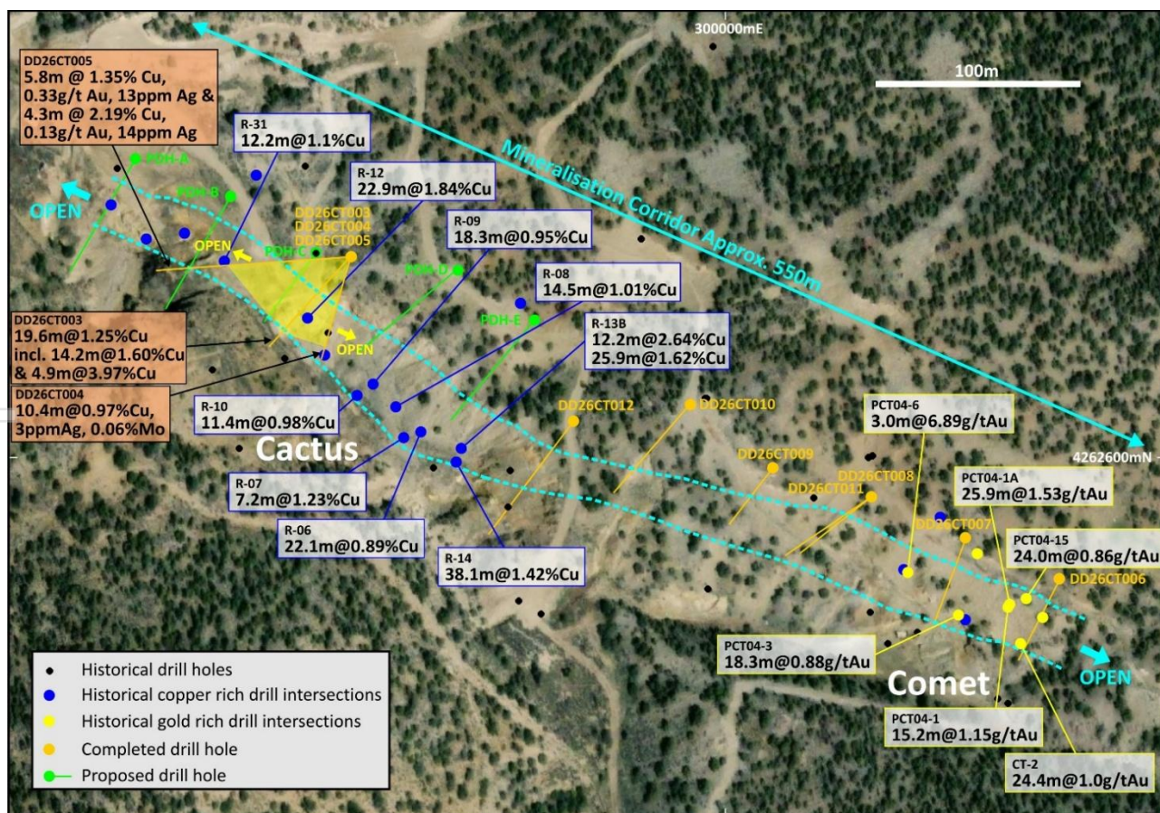
Figure 2: Location of Hawk drill holes DD26CT006-012 and historical shallow drill hole intersections.
