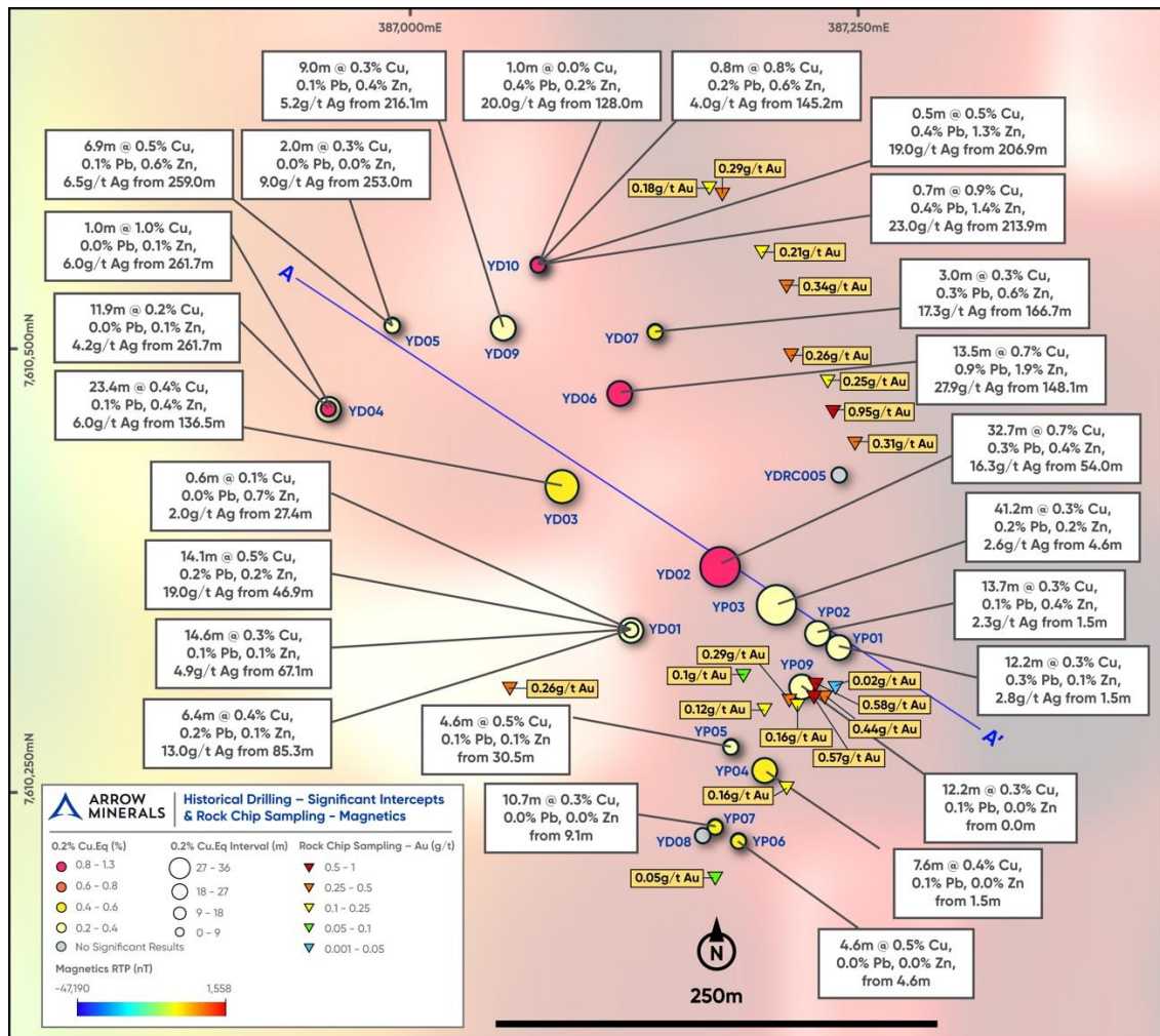
Figure 3. Yarraloola Mine Prospect: Historical drilling significant intercepts shown with rock chip samples with gold analyses overlain on TMI-RTP magnetic image Coordinate system: MGA2020 Zone 50 [EPSG: 7850]
