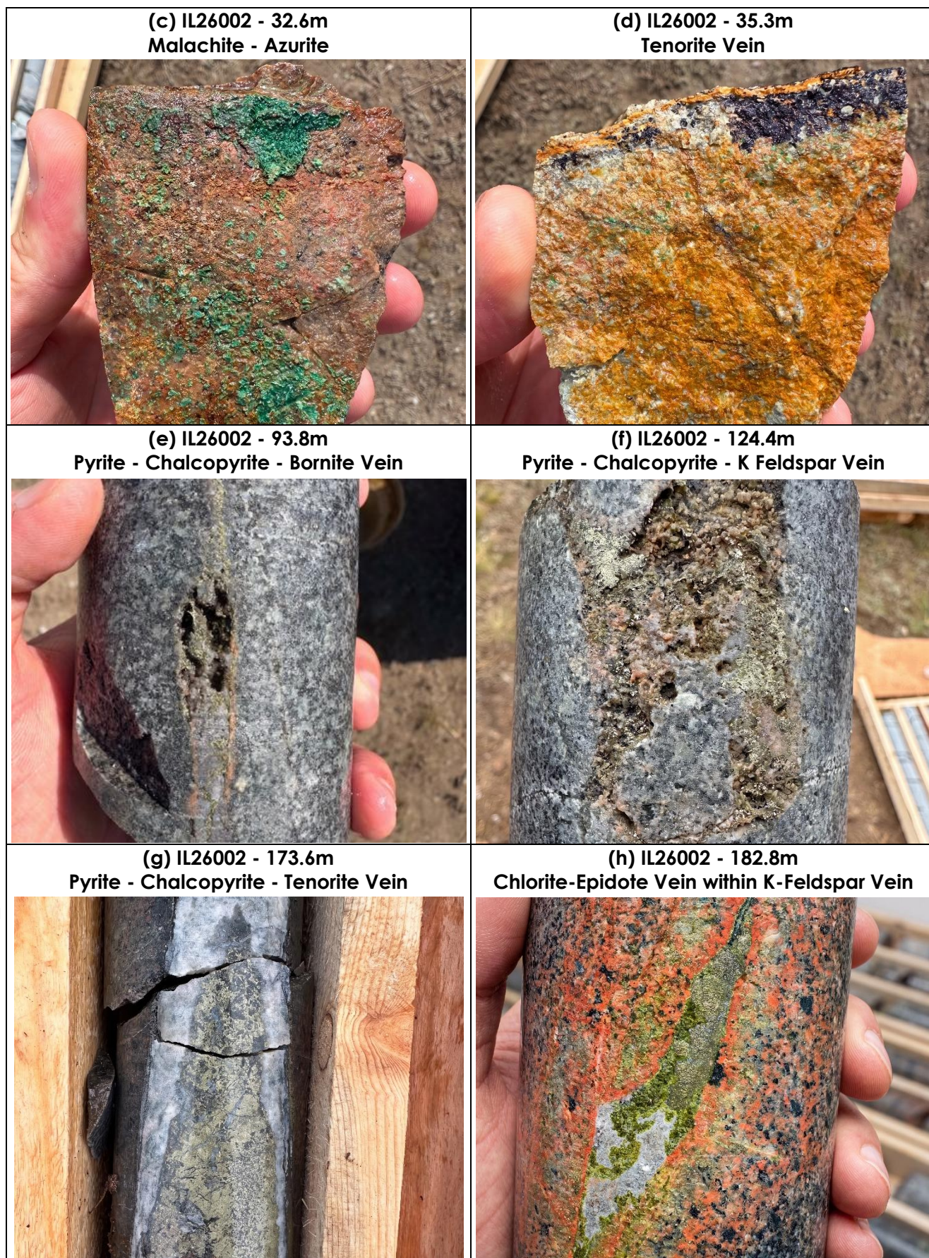
Figure 3 - Typical mineralisation and veining at Ilksan in hole DDH-IL26002
