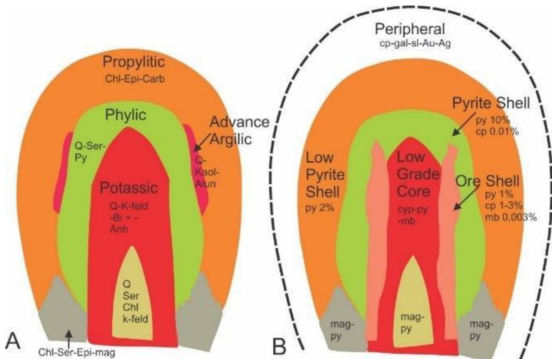
Figure 5 - Ore deposit model adapted from Lowell and Gilbert 1970.
