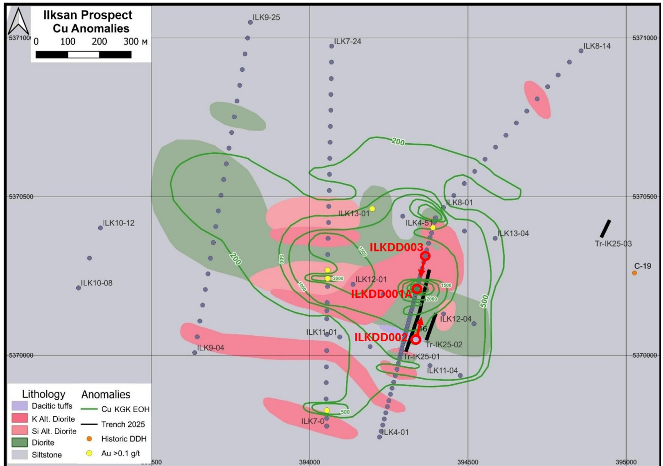
Figure 2 – Lithology map with copper and gold anomalism of the Ilksan Prospect at Baynazar. Completed diamond drill holes are annotated in red.
