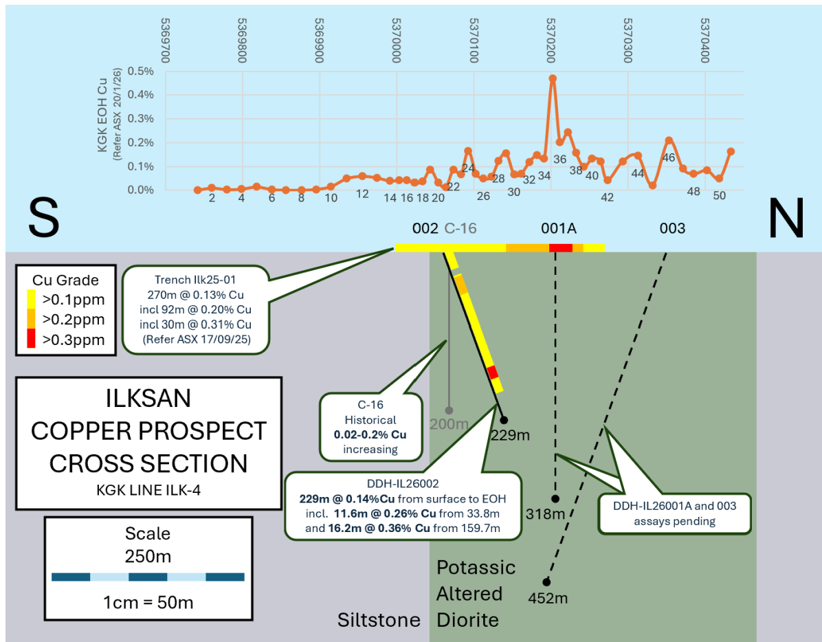
Figure 4 – Cross Section at Ilksan. Geological Interpretation to be added with results of additional holes.
