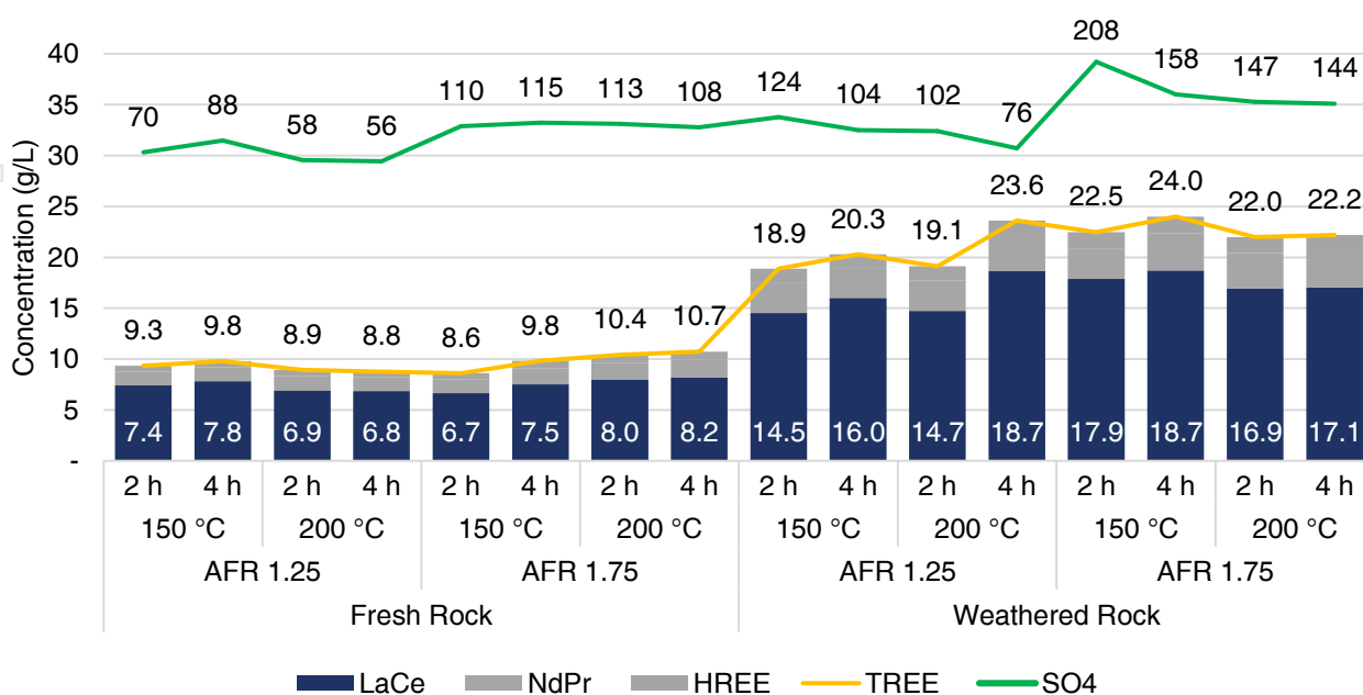
Figure 79: TREE and SO4 Concentrations in the PLS (g/L) - Sulista Weathered and Fresh Rock
