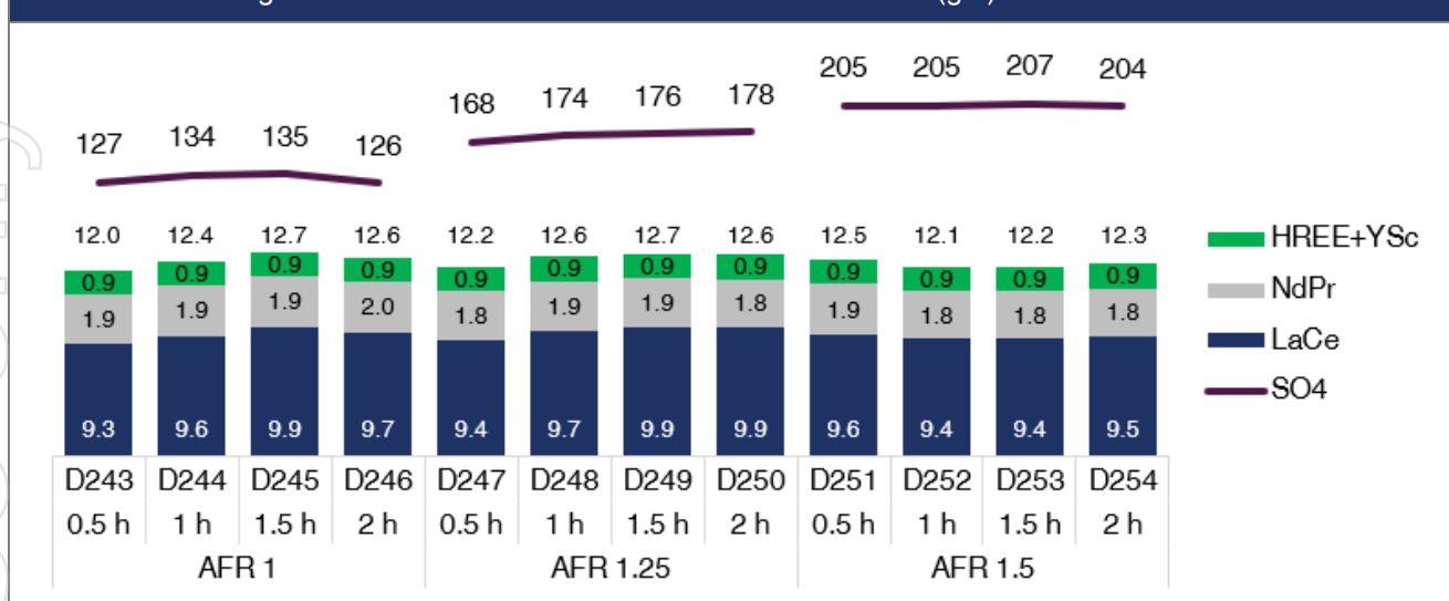
Figure 68: TREE and SO 4 Concentrations in the PLS (g/L) – Monte Alto CAB
