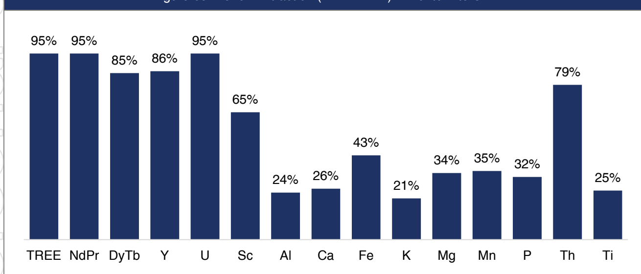
Figure 69: Bench Extraction (AFR 1 – 1h) – Monte Alto CAB
