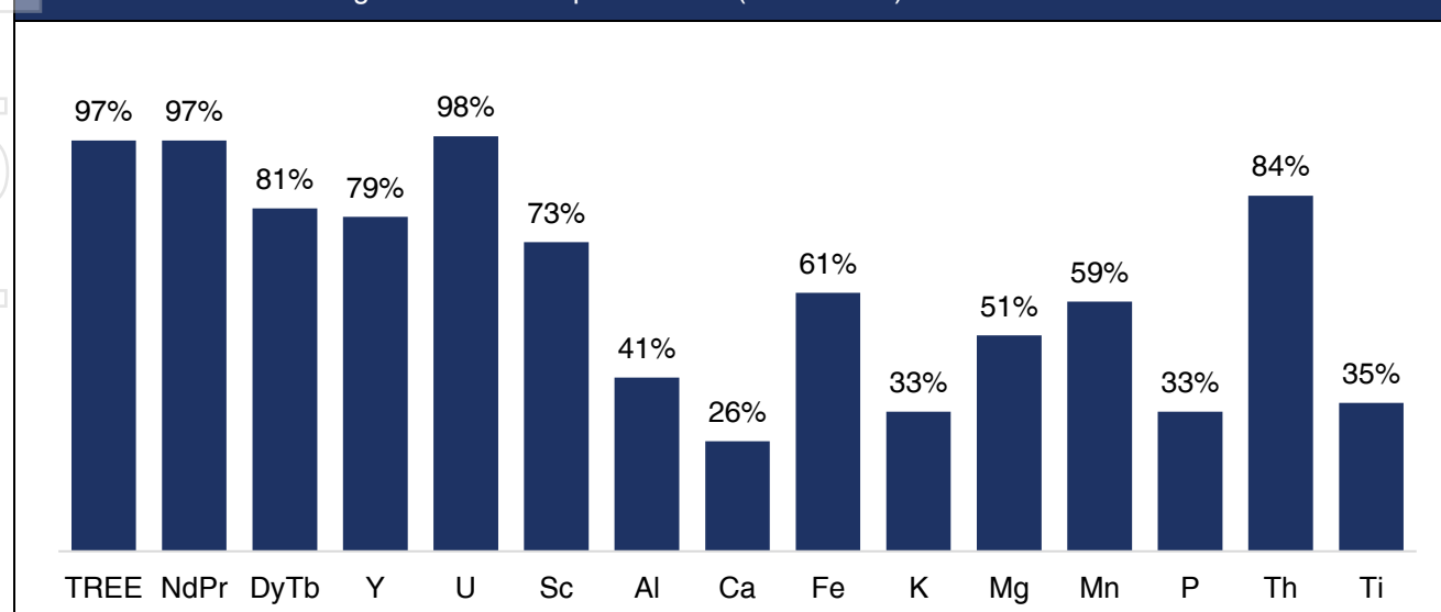
Figure 70: Scale-Up Extraction (AFR 1 – 1h) – Monte Alto CAB
