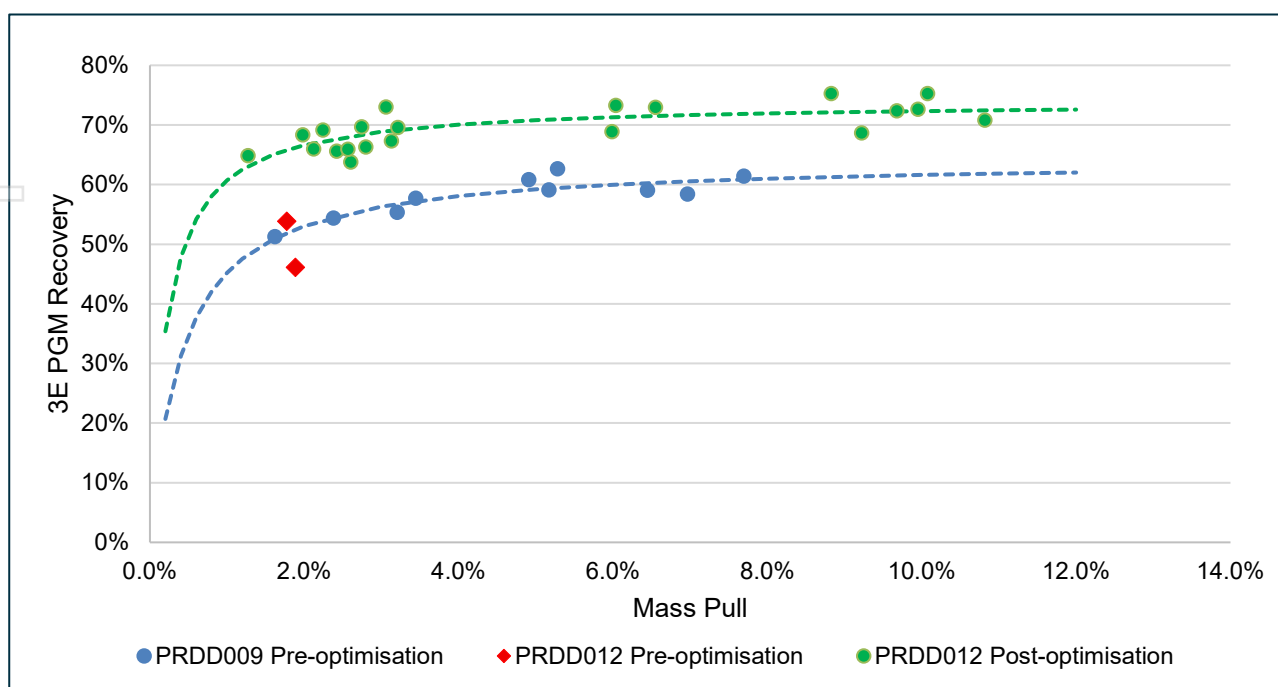
Figure 3: Flotation Recovery vs Mass Pull (Pre- and Post-Optimisation)
