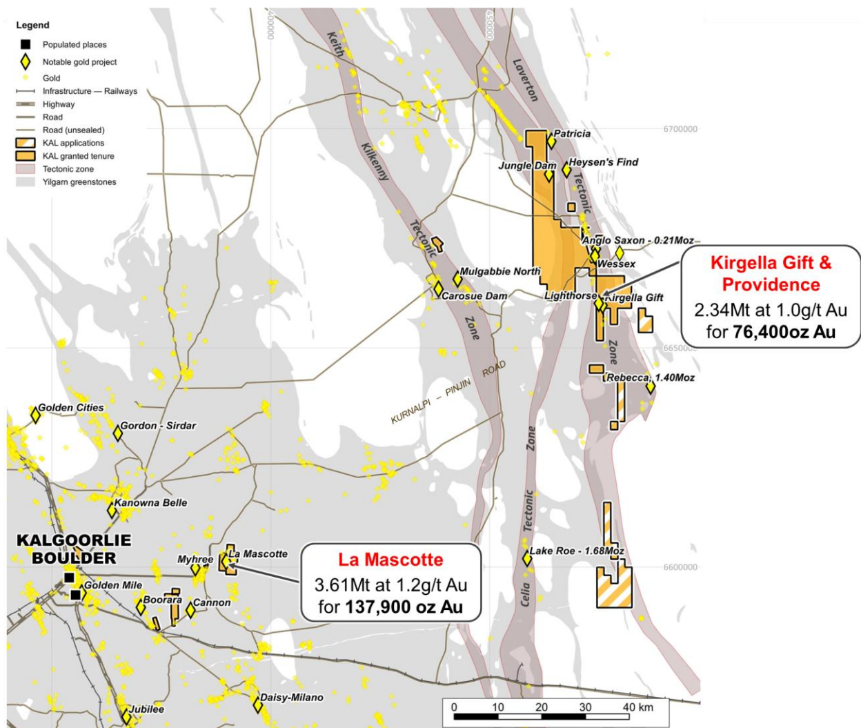
Figure 1 – Location map of the Kirgella Gift-Providence gold deposit and the Lighthouse prospect within KalGold's Pinjin Project, located around 140 km northeast of Kalgoorlie-Boulder. The project is situated approximately 25 km north of Ramelius Resources' (ASX: RMS) Rebecca Gold Project. Also shown is KalGold's outcropping La Mascotte gold deposit 35 km east of Kalgoorlie. Projection: MGA 94 Zone 51.
