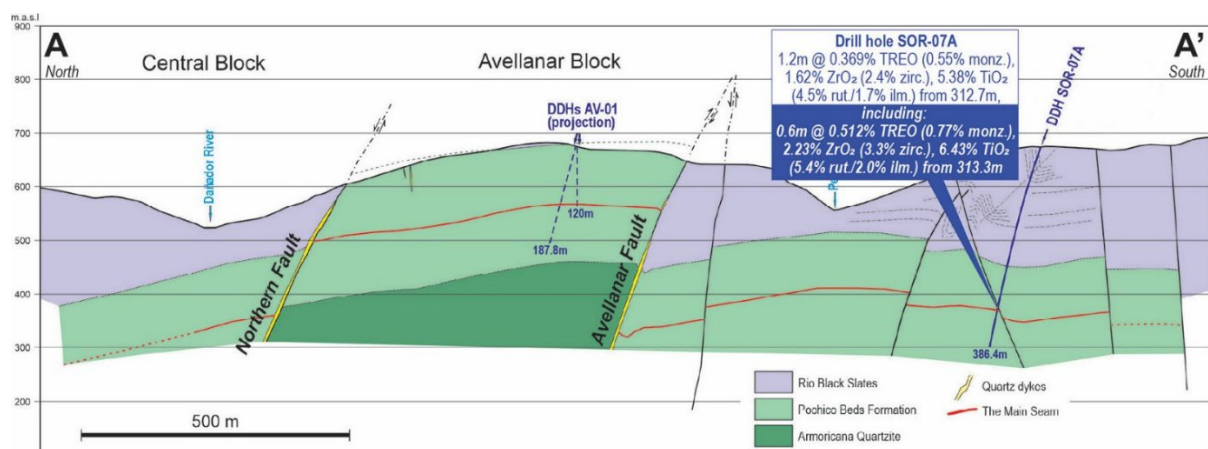
Figure 3 – SOR-07A cross-section.
