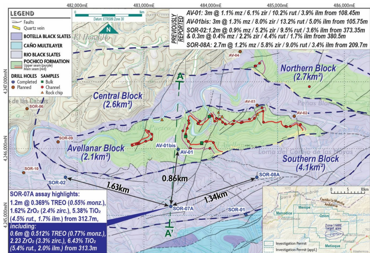
Figure 2 – Map showing location of drill holes and channel samples with assay highlights 7 . Location of cross-sections A – A' (Figure 3) highlighted.
