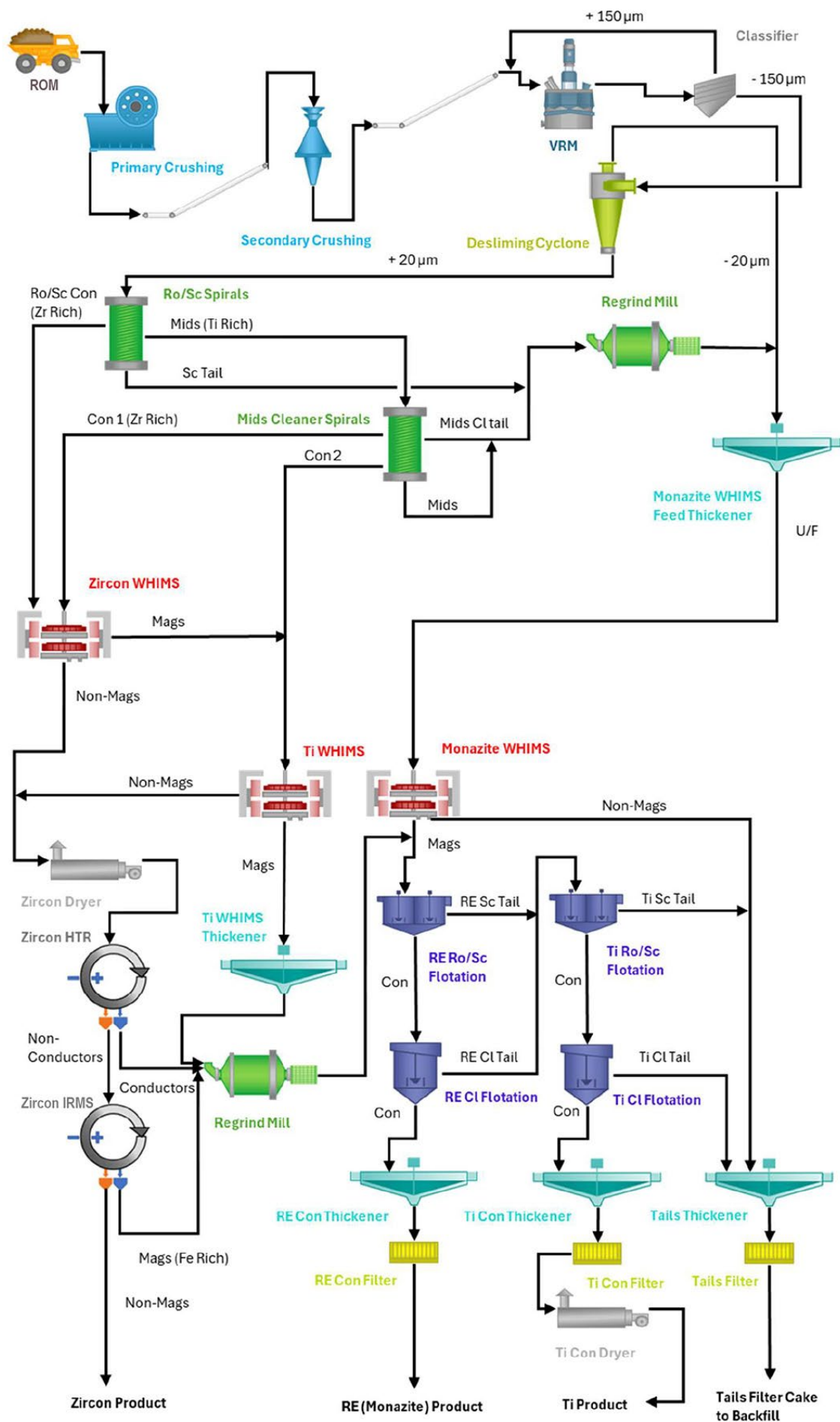
Figure 5 - Orión Project processing flowsheet block flow diagram.
