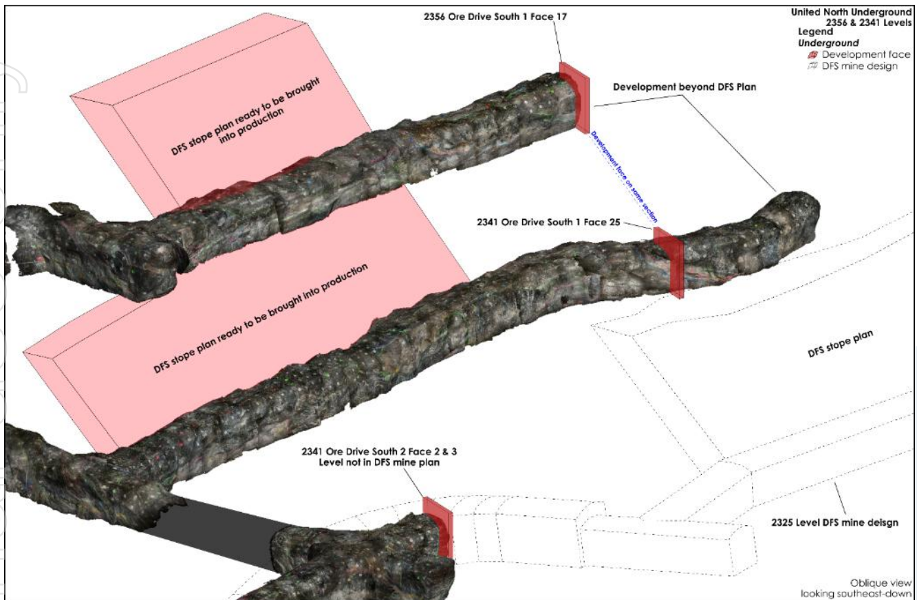
Figure 4 – United North 2356 & 2341mRL ore drives south with DFS mine plan, oblique view looking down to the southeast
