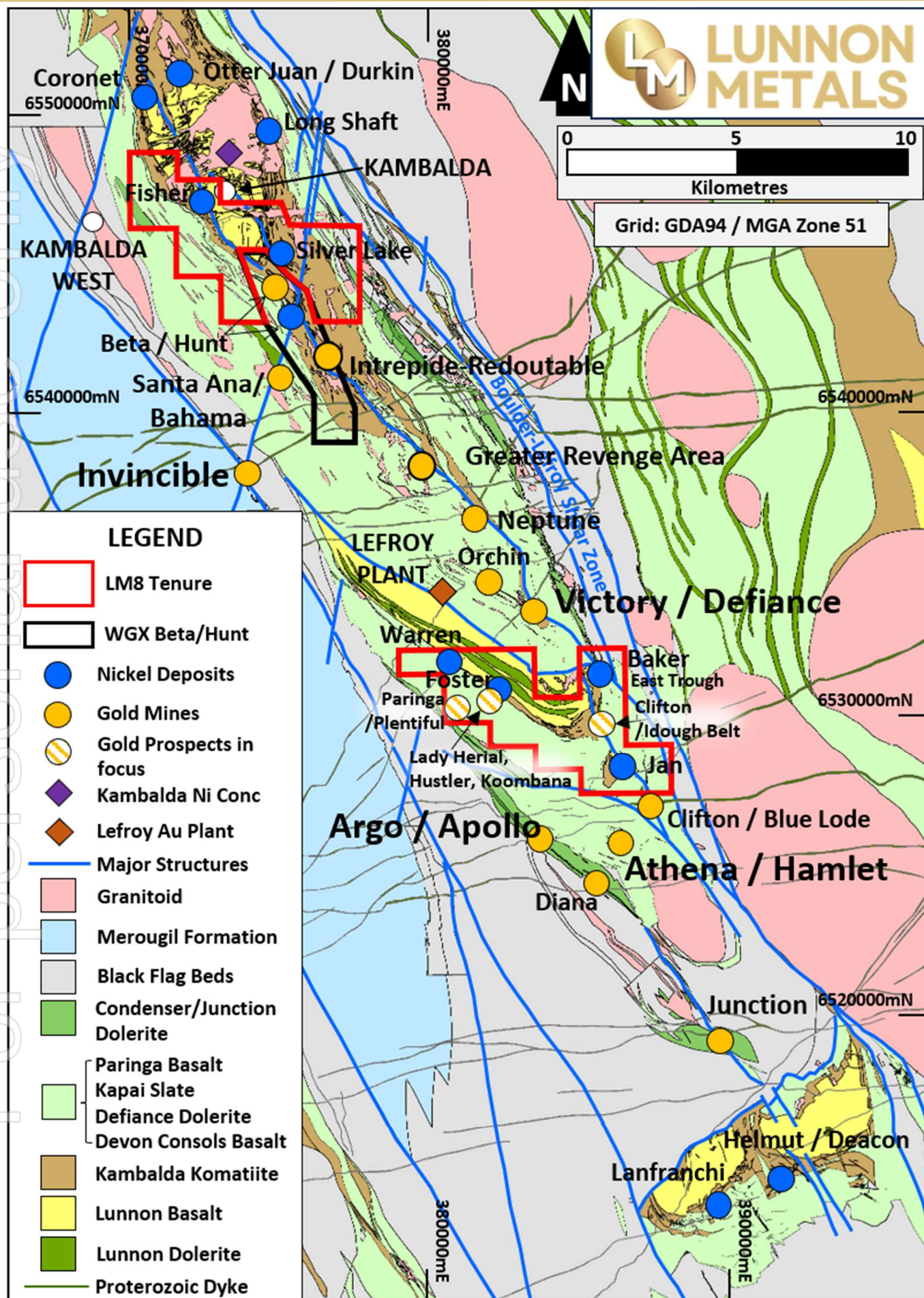
Figure 7: Location of the KGNP (red outlines) at the local Kambalda Nickel District / St Ives Gold Camp scale; showing surface geology and structure of this significant Australian gold camp.
