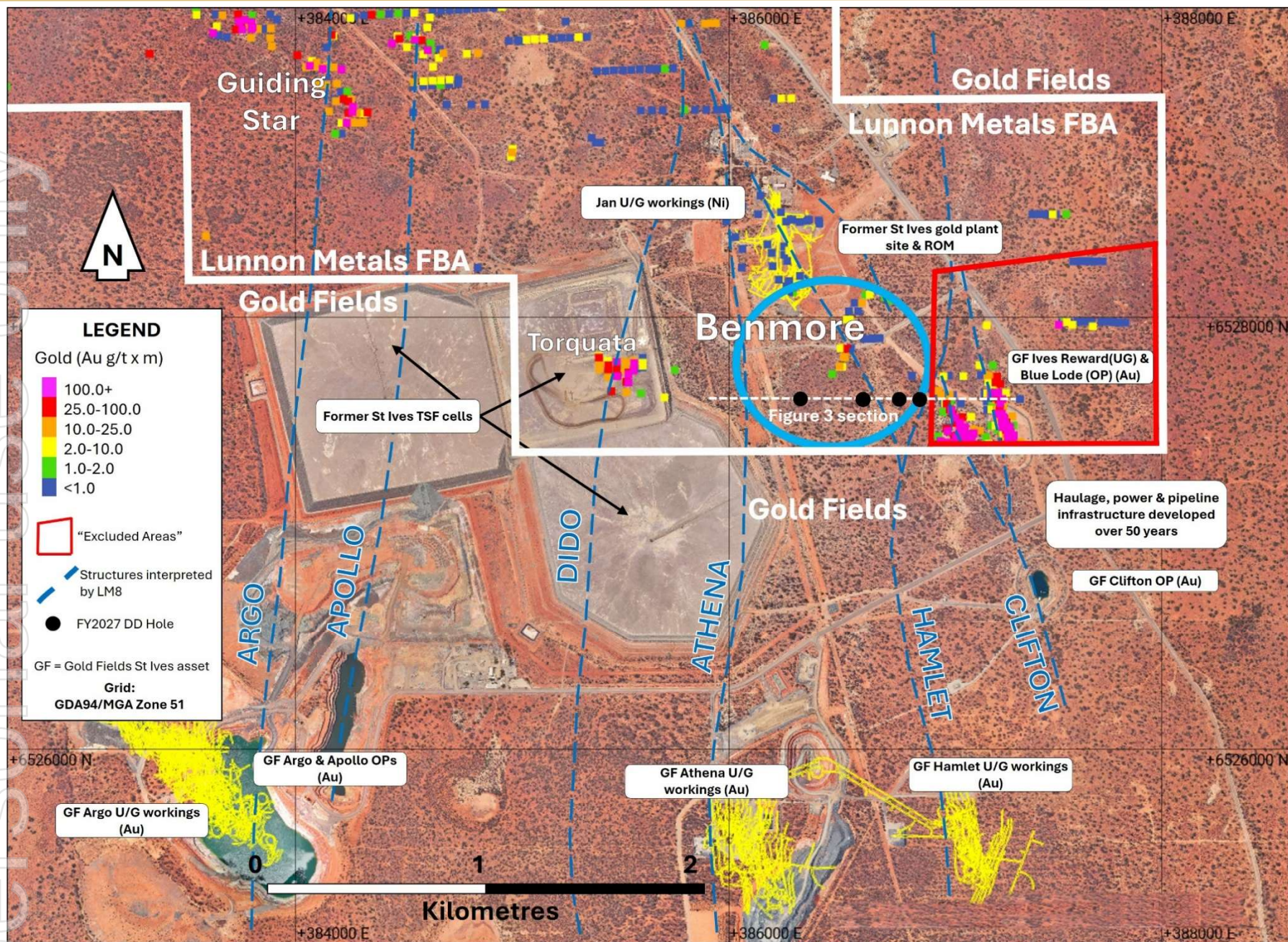
Figure 2: Plan view of the Benmore target area showing the location of the DD transect, the Jan underground nickel mine and the nearby underground gold mines on Gold Fields’ leases to the south.
