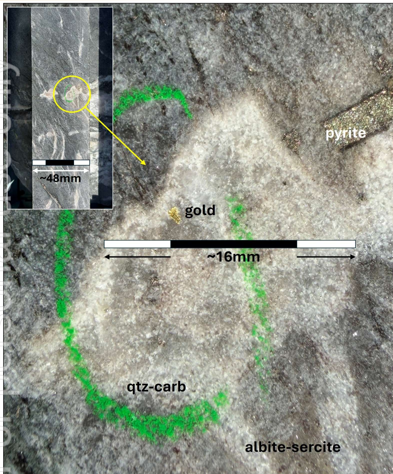
Figure 6: Zoomed image of DD core at 302.25m from JAN26DD_011, illustrating observed visible gold in an interval that assayed only 0.92 g/t Au.
