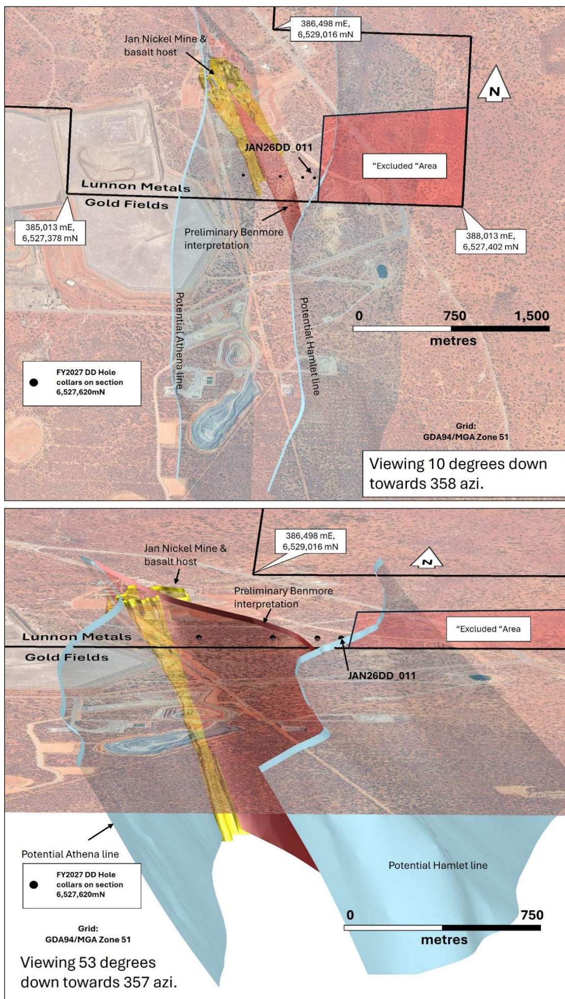
Figure 4: Isometric views of preliminary structural interpretation of structures at Benmore
