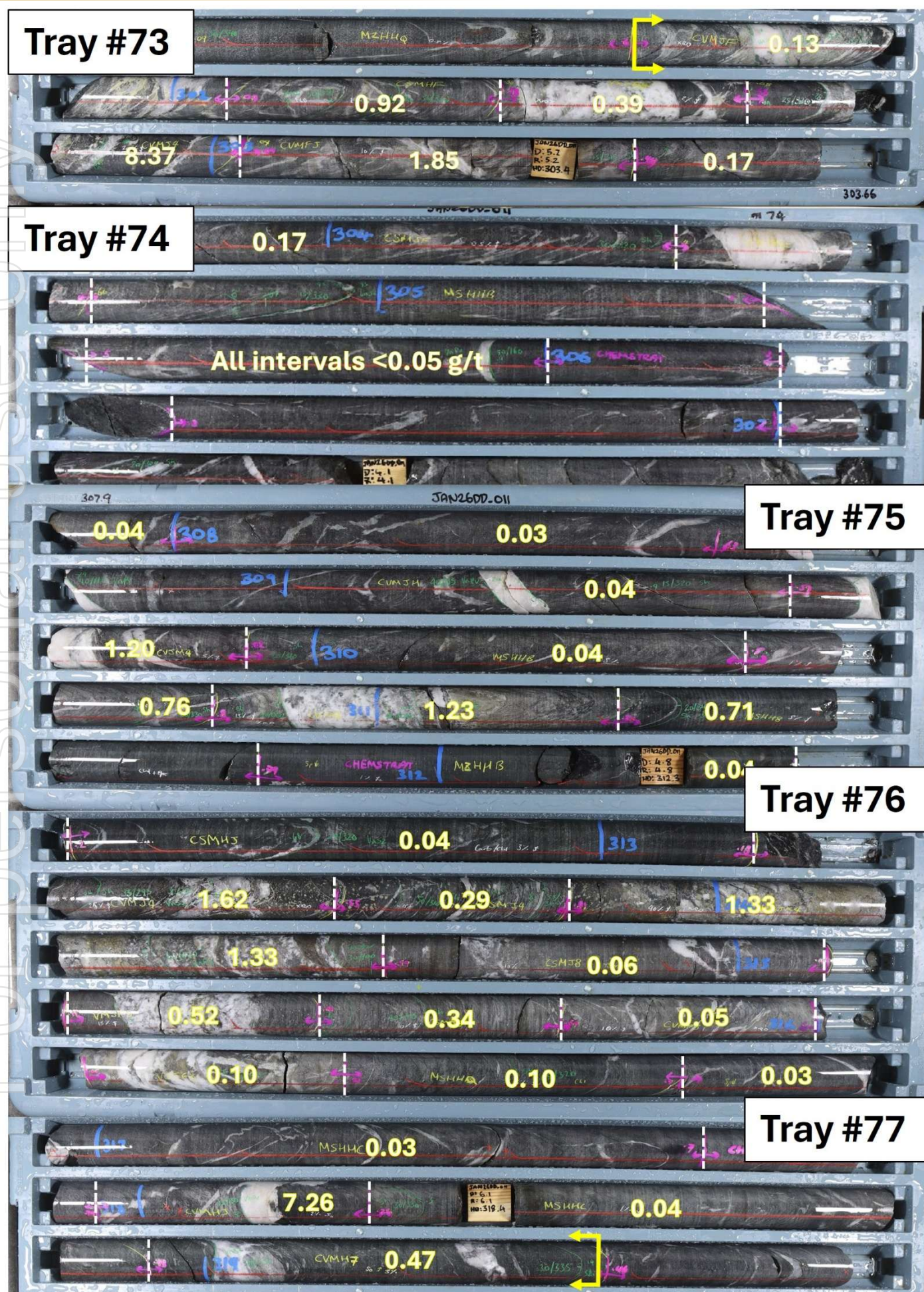
Figure 5: DD core trays from JAN26DD_011 showing sheared, foliated biotite altered mafic rock with zones of albite-pyrite rich breccias and veins. Sampled intervals are shown with the relevant returned assays in g/t Au (Annexure 2 also details individual interval assays).
