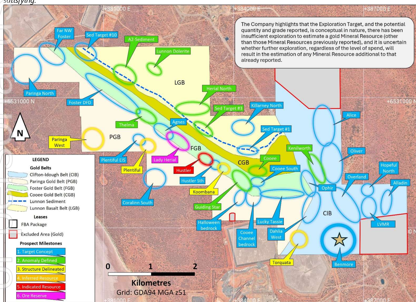
Figure 1: Plan view of the FBA showing the interpreted gold belts hosting the current portfolio of gold targets, ranging in maturity from Conceptual to Resource Definition. Benmore is in the south-east corner of the portfolio.
