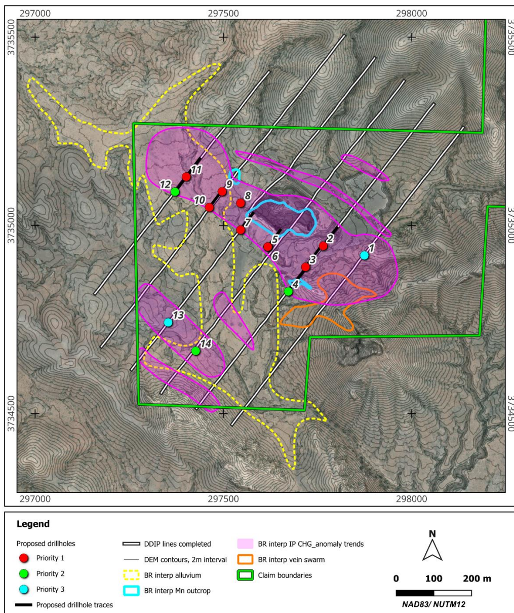
Figure 1. Black Rock Manganese Mine Prospect – Geophysical IP Survey Data Interpretation
