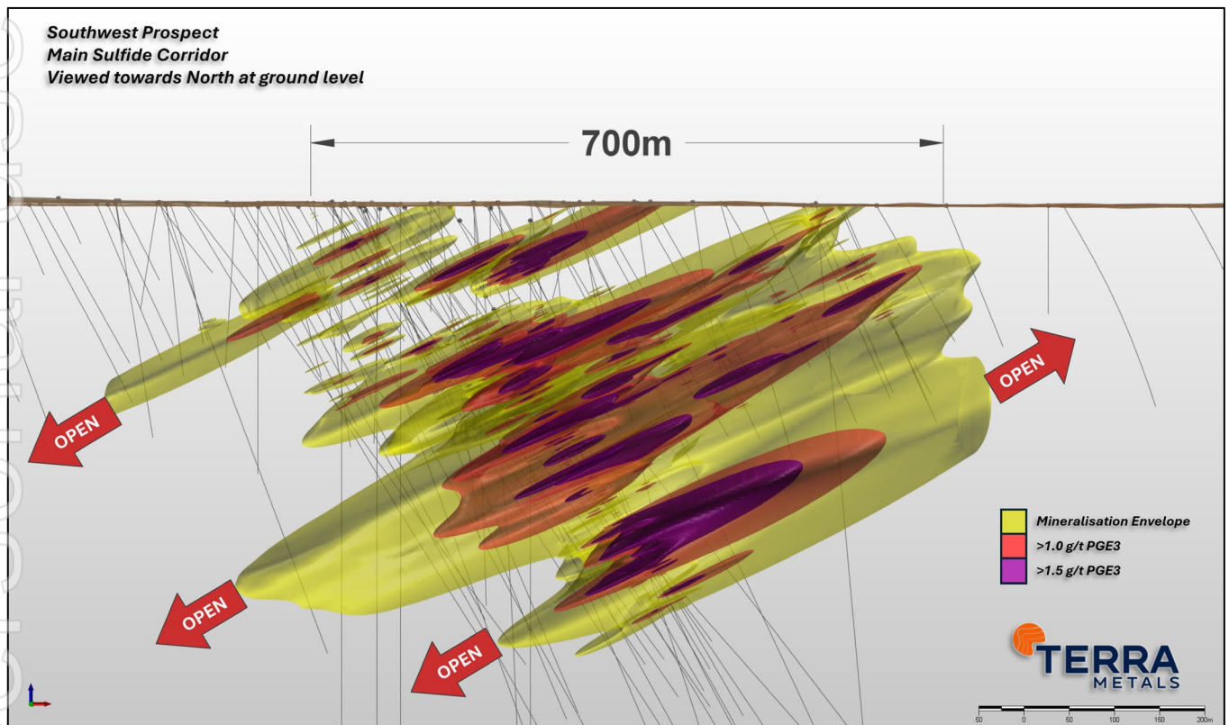
Figure 4. 3D view of Southwest Project viewed from the South, showing Mineralisation envelope and high-grade reefs interpreted from current drill results.
