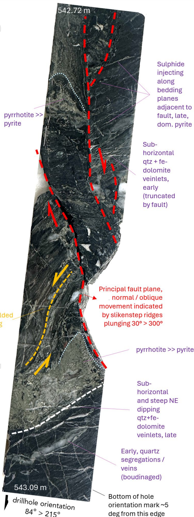
Figure 1: MD002DD half HQ core from 542.72 to 543.09 m depth simulating a vertical section looking approximately WNW with core tilted to mimic the as-drilled orientation. The interval is cut by a fault (principal slip planes in red) with normal movement indicated by slickenstep ridges. A pyrrhotite-dominant sulphide assemblage is hosted within the fault, and sulphide is also hosted along bedding planes adjacent to the fault. Multiple generations of veining and mineralisation are evident. Fault hosted sulphide mineralogy identified by binocular microscope examination is pyrrhotite-dominant with subordinate pyrite. Early magnetite in the wall rock is destroyed within the vein and fault gouge. Sample HQ2652 over this interval returned 0.239 g/t Au, 1,630 ppm Cu, 6.70% S, 15.05% Fe, 300 ppm As, 11.15 ppm Bi and 1.61 ppm Ag. The sample is estimated to contain approximately 11 to 16% pyrrhotite, 1 to 5% pyrite, 0.5% chalcopyrite and 0.1% arsenopyrite by weight. These mineral abundances have been estimated by mass balance from the whole-rock assay – the method and limitations are set out in JORC Table 1, Section 2, Other exploration data. Magnetite is estimated at less than 0.05% by weight, consistent with magnetic susceptibility measurements. This fault orientation (steep to the NNE), and the associated kinematics are consistent with the proposed negative flower structure framework (Figure 6). Within this preliminary framework the modelled conductor (dipping steeply to the SSW) forms at a complementary bounding wall to the flower structure.
