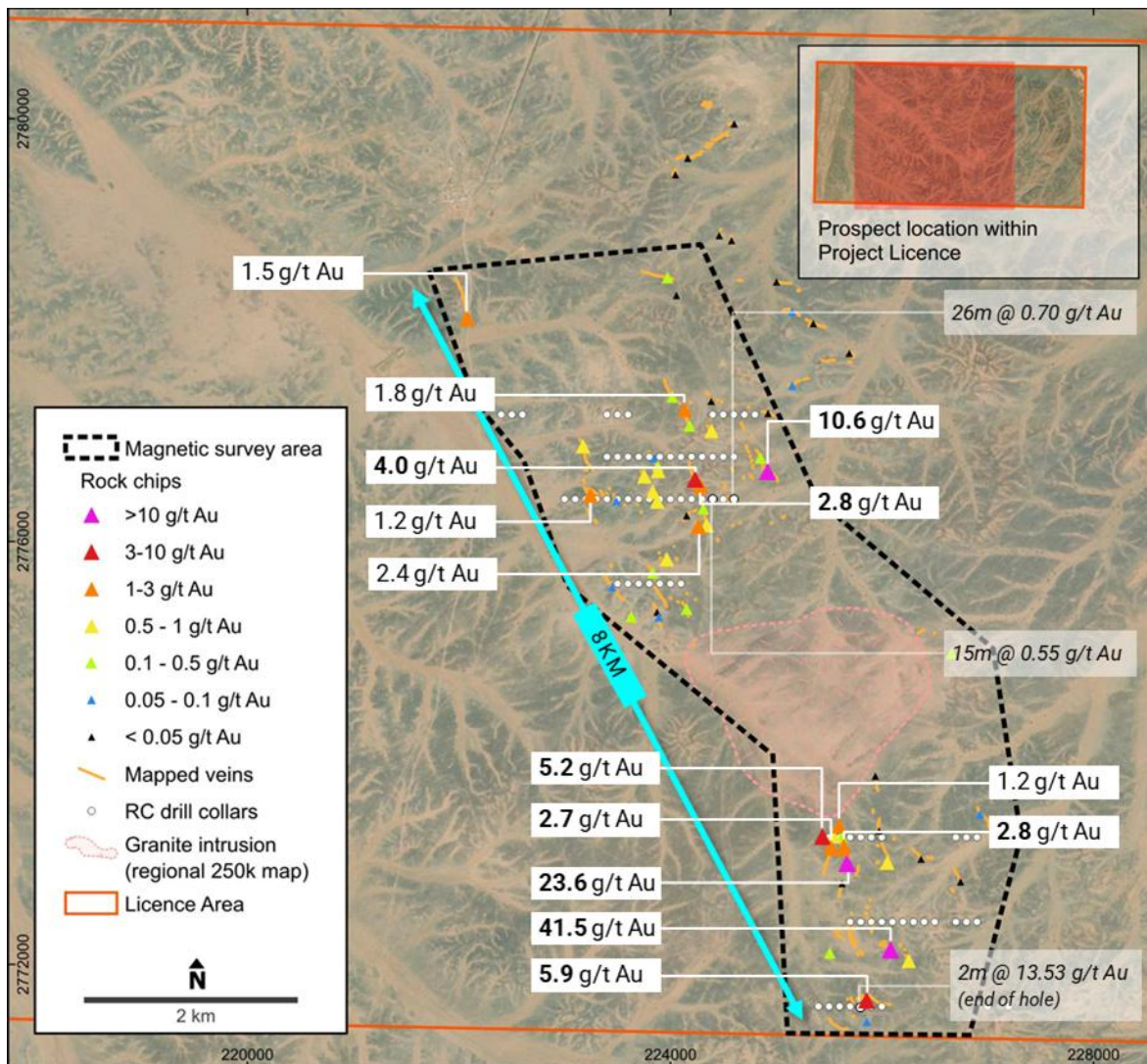
Figure 3 Magnetic survey area at Wadi Jarir target area
