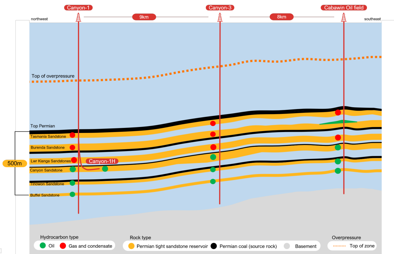
Figure 2: Six reservoir intervals, hydrocarbon distribution and inferred top of overpressure (not to scale)
