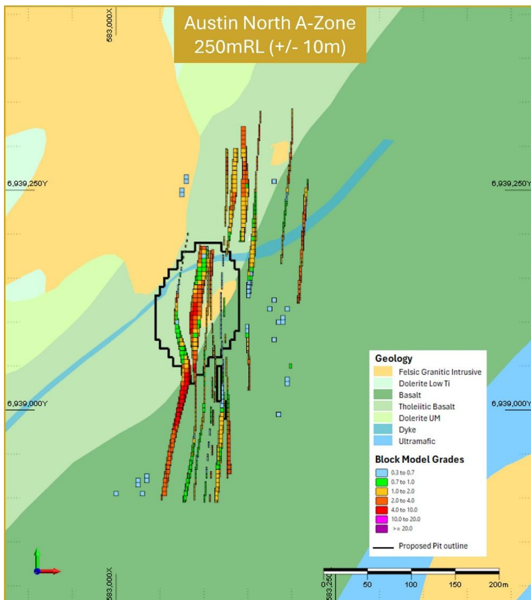
Figure 18: Plan view section of A-Zone basement geology (transported cover and oxides removed)
