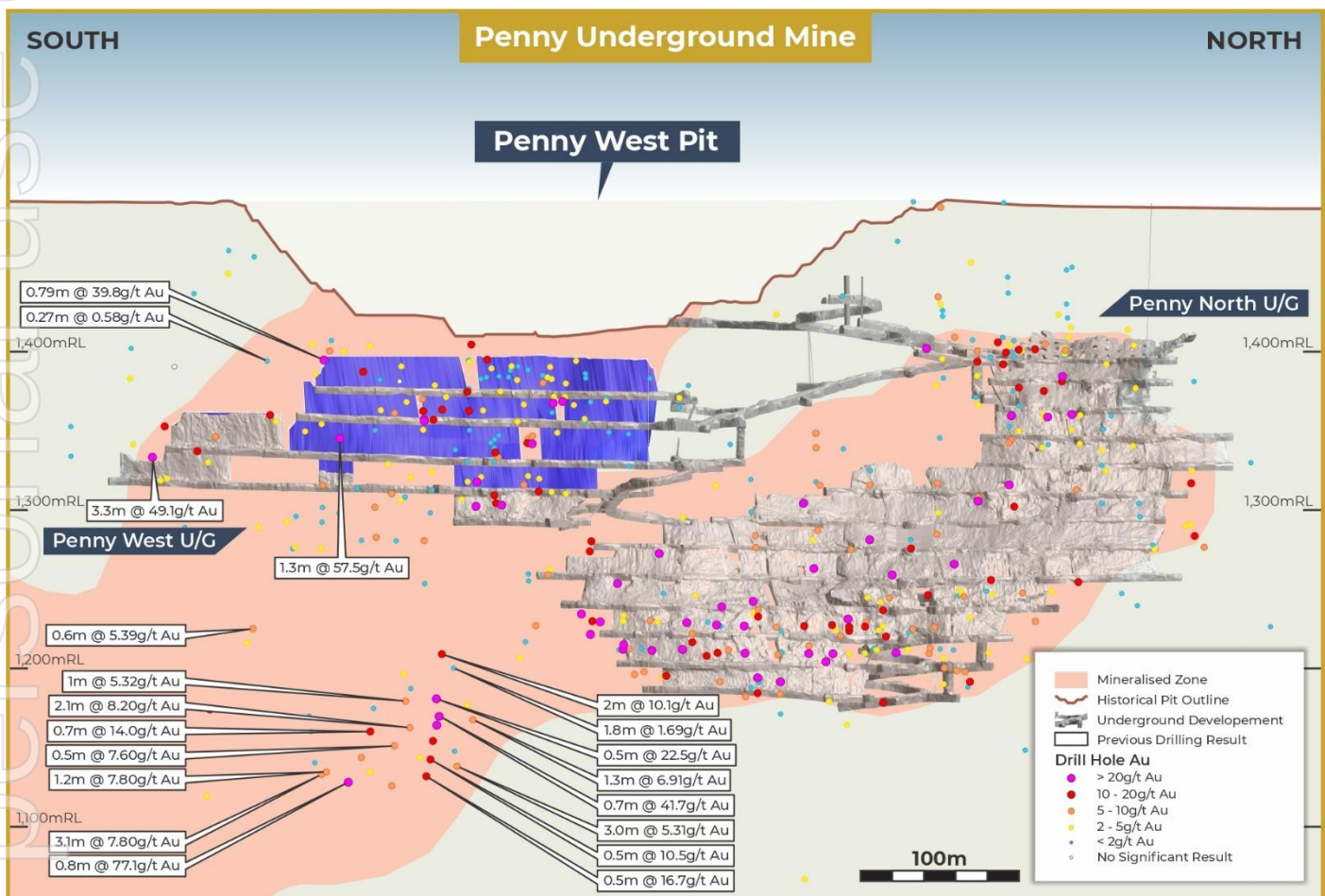
Figure 24: Penny longsection with remaining stopes to be mined at Penny West
