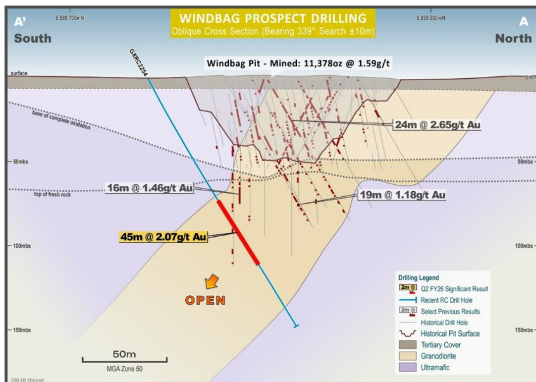
Figure 10: Windbag – cross section A' - A showing recent result
