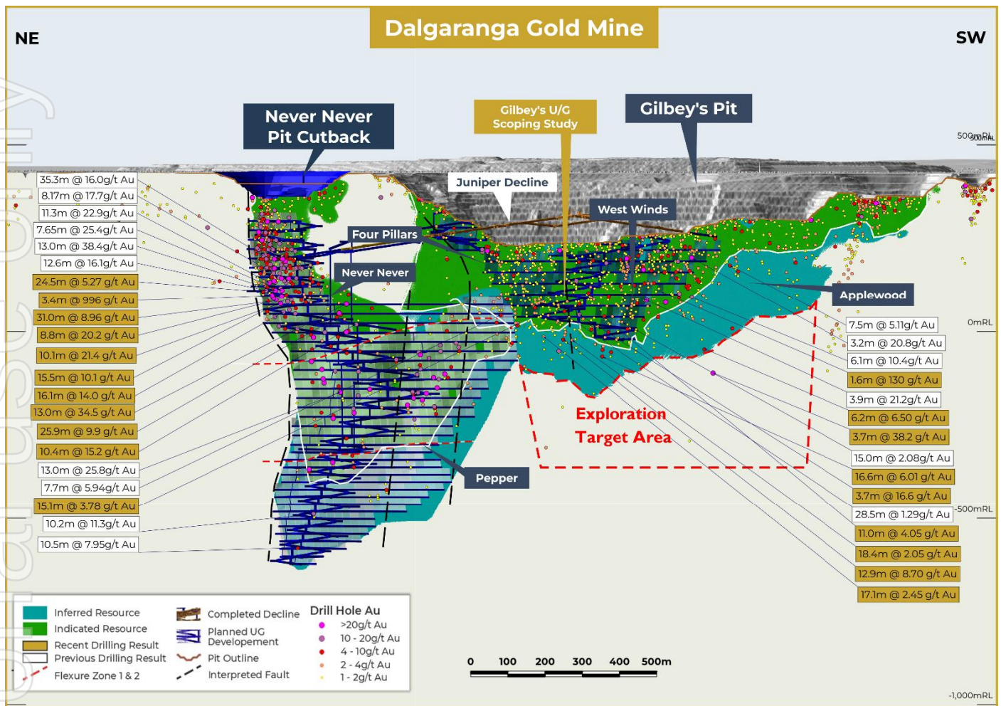
Figure 23: Dalgara longsection of Mineral Resources with Gilbey's Underground Exploration Target area
