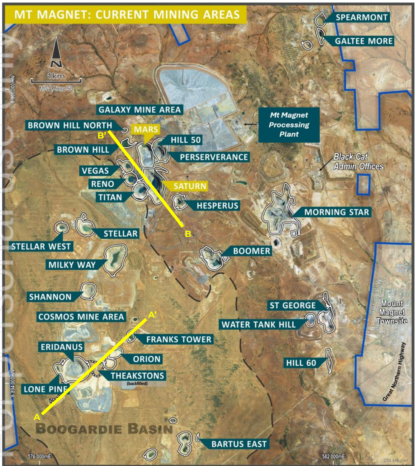
Figure 3: Mt Magnet mining locations. Section lines for Eridanus mine area (A – A') and Galaxy mine area (B – B') in yellow
