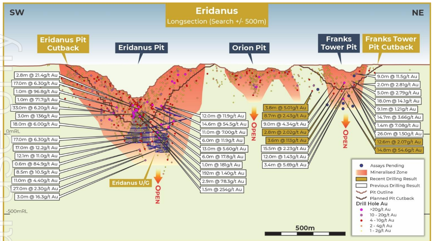
Figure 12: Eridanus - Franks Tower long section facing northwest with previously released drill results (see RMS ASX release 'Exploration Update', 22 July 2026)
