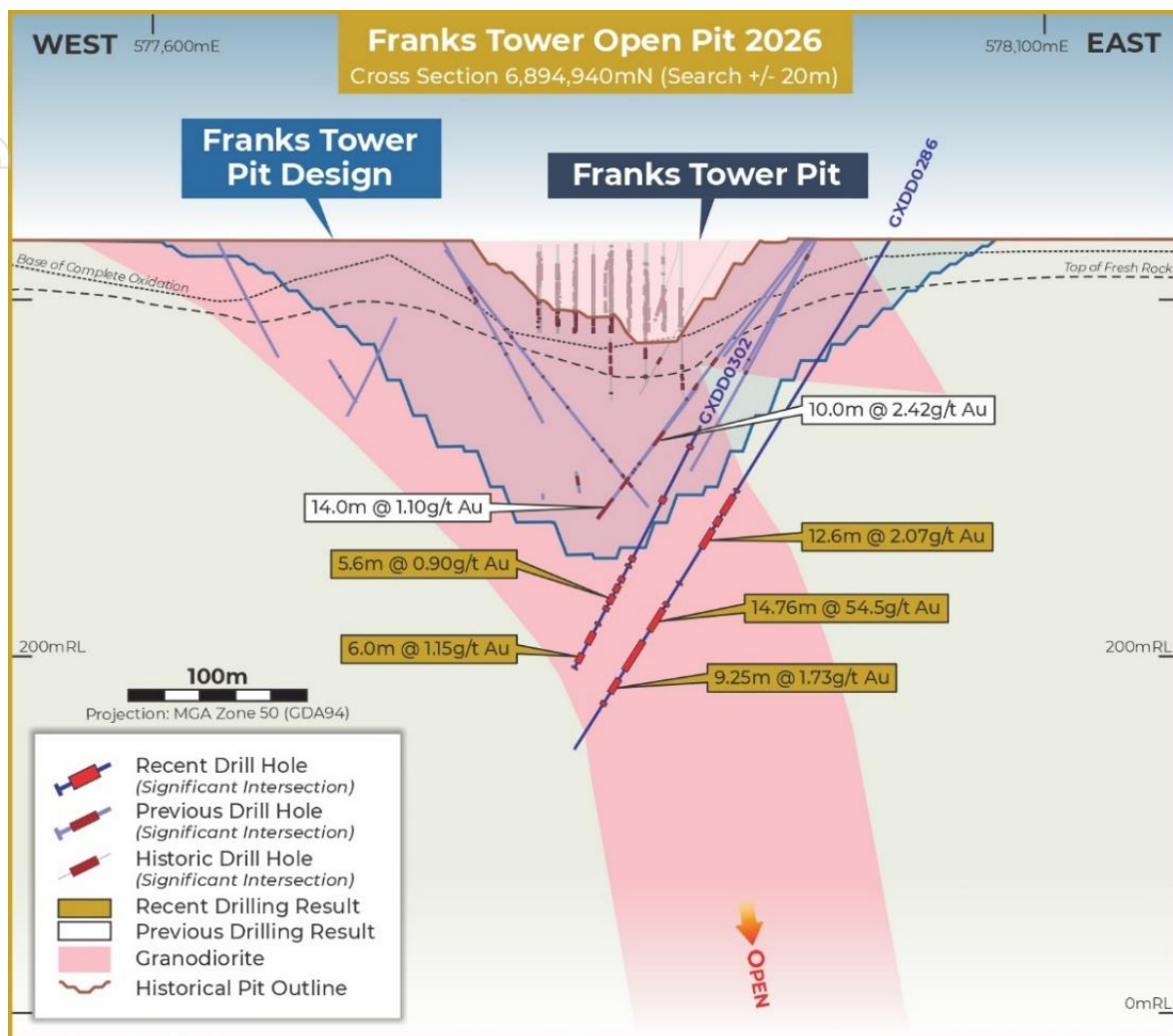
Figure 14: Franks Tower – cross section showing recent results
