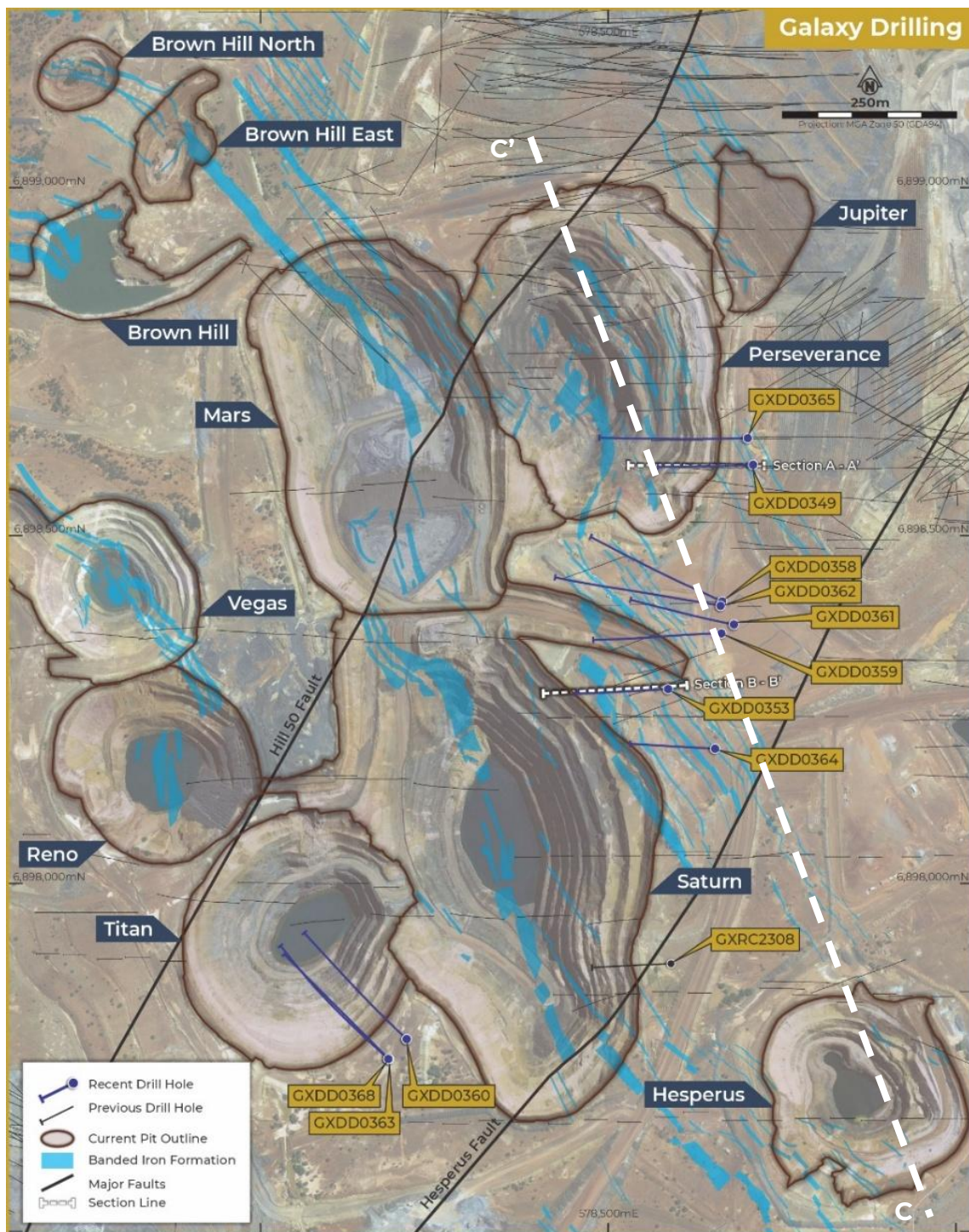
Figure 5: Galaxy mine area – plan view showing drill hole locations at Perseverance South and Titan
