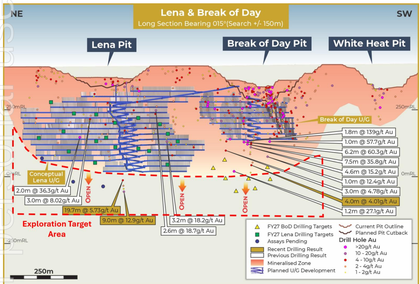
Figure 16: Lena-Break of Day long section with conceptual Lena underground and Exploration Target Area
