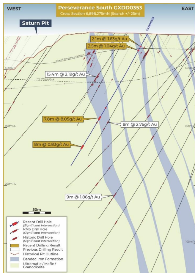
Figure 7: Perseverance South - cross section B-B' showing recent results
