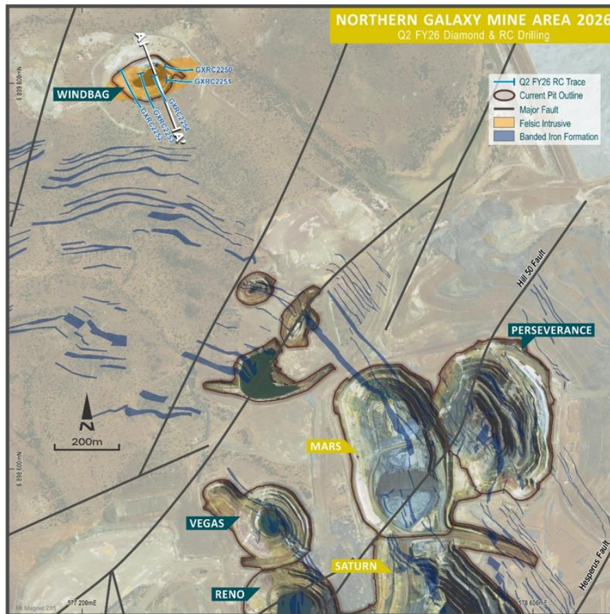
Figure 9: Windbag – location map
