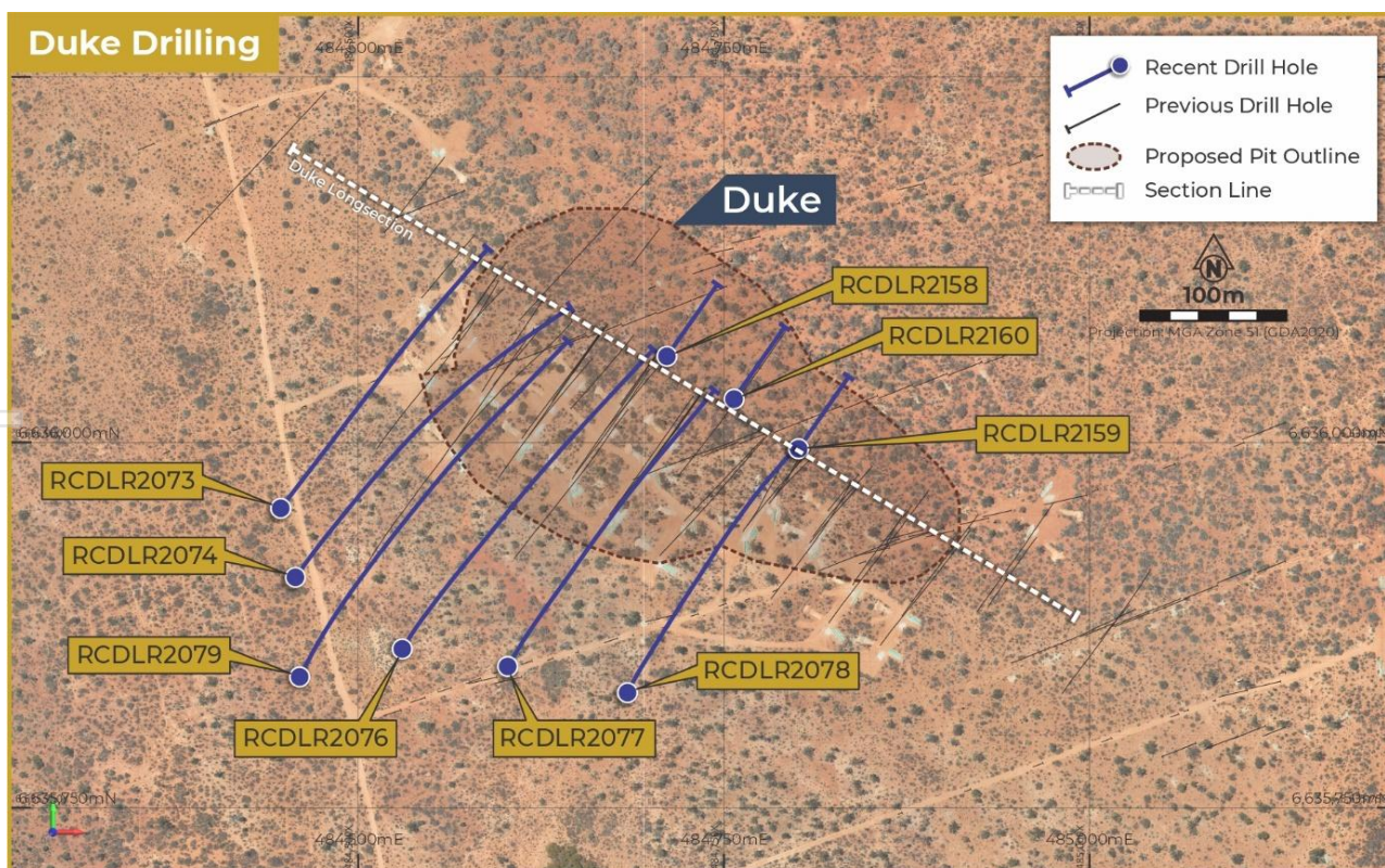
Figure 27: Duke - drill hole location plan
