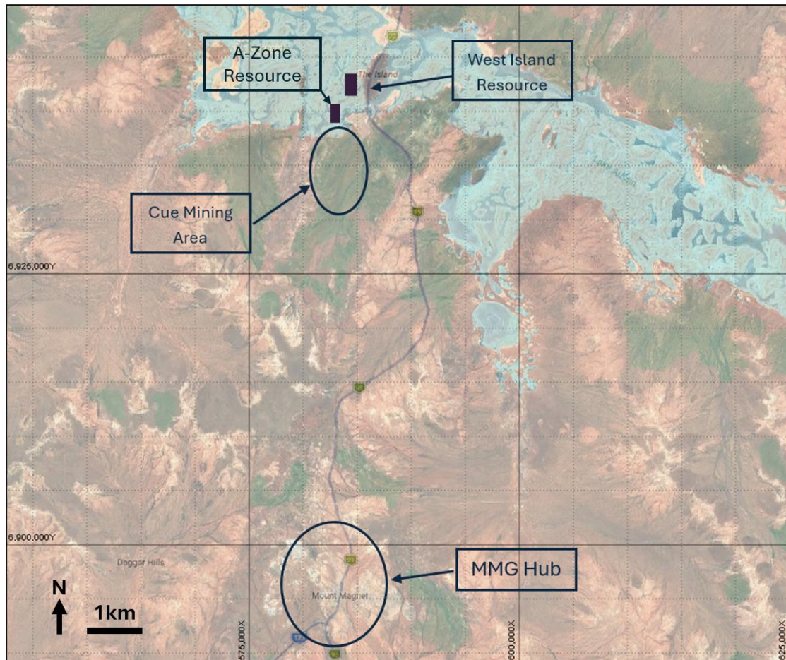
Figure 17: Location map of the Lake Austin deposits, Cue Mining Area, and Mt Magnet
