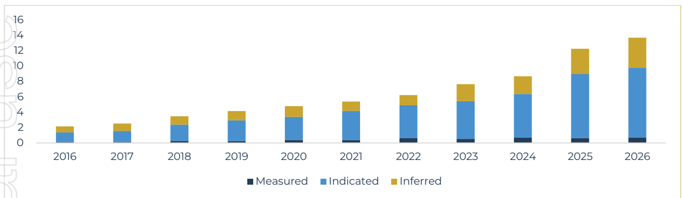
Figure 30: Historical Mineral Resources (Moz)
