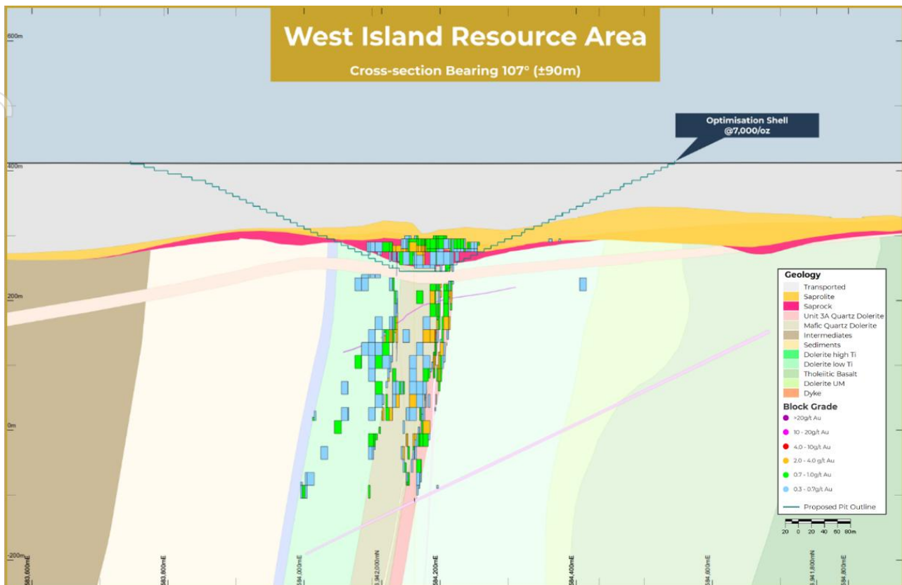
Figure 21: Cross section of West Island geology displaying cover, supergene, and fresh rock mineralisation
