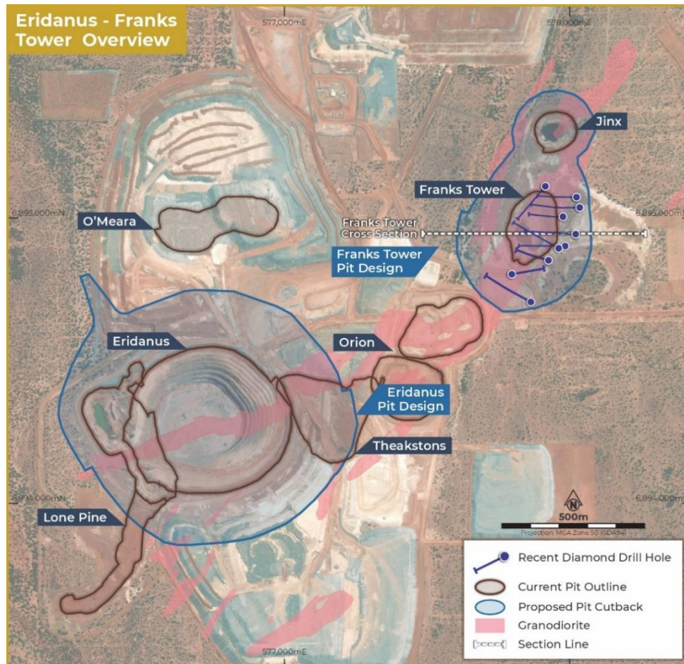
Figure 13: Eridanus to Franks Tower 2km long corridor showing modelled granodiorite intrusive
