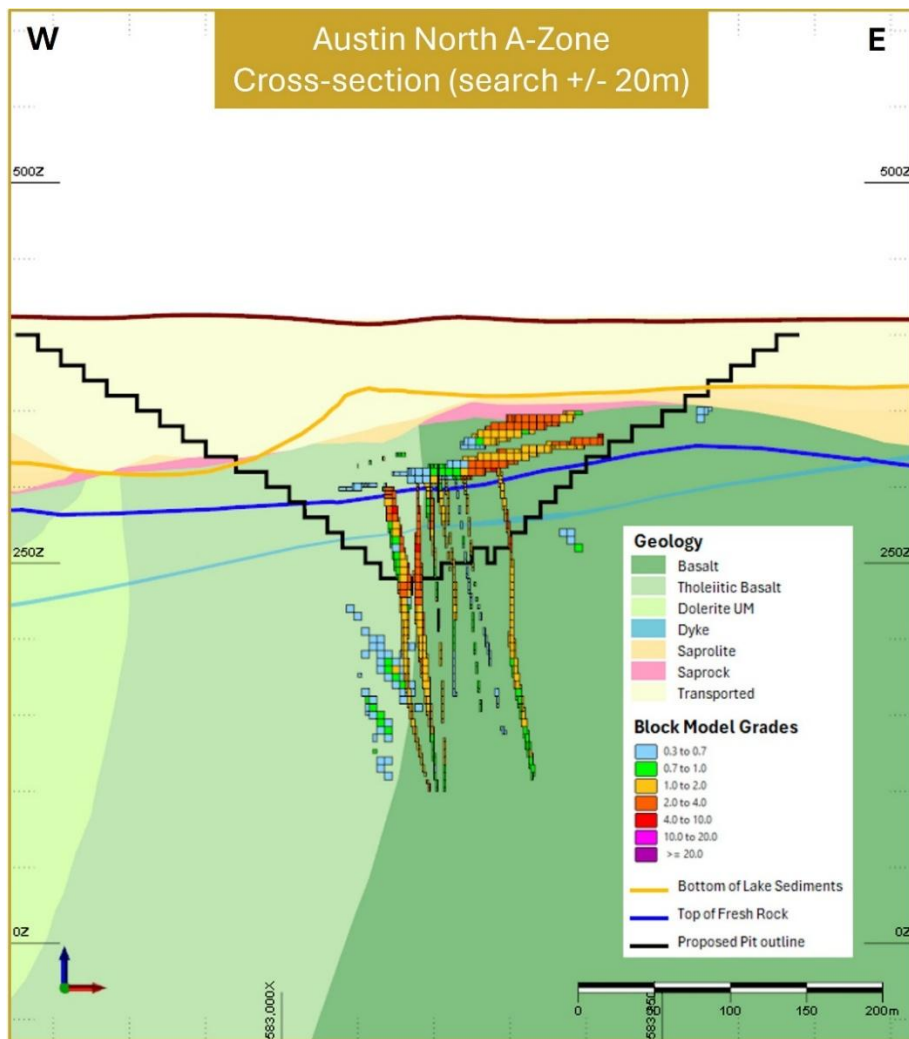
Figure 19: Cross section of A-Zone geology displaying cover, supergene, and fresh rock mineralisation
