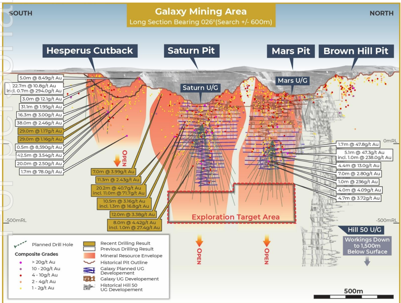
Figure 4: Galaxy Group mining area 2km long corridor
