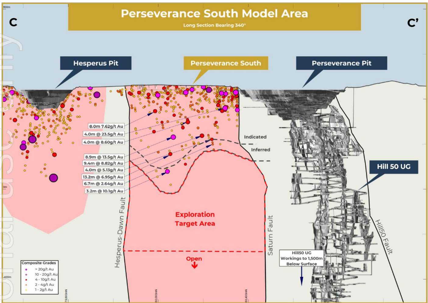
Figure 8: Perseverance South resource area and Exploration Target facing southwest (C – C' Figure 4)
