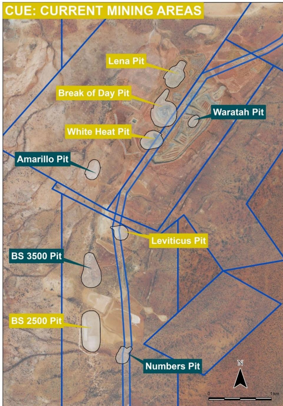
Figure 15: Cue current mining locations
