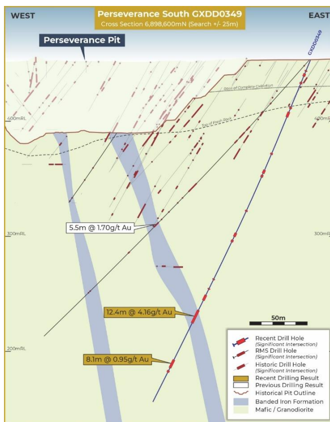
Figure 6: Perseverance South - cross section A-A' showing recent results
