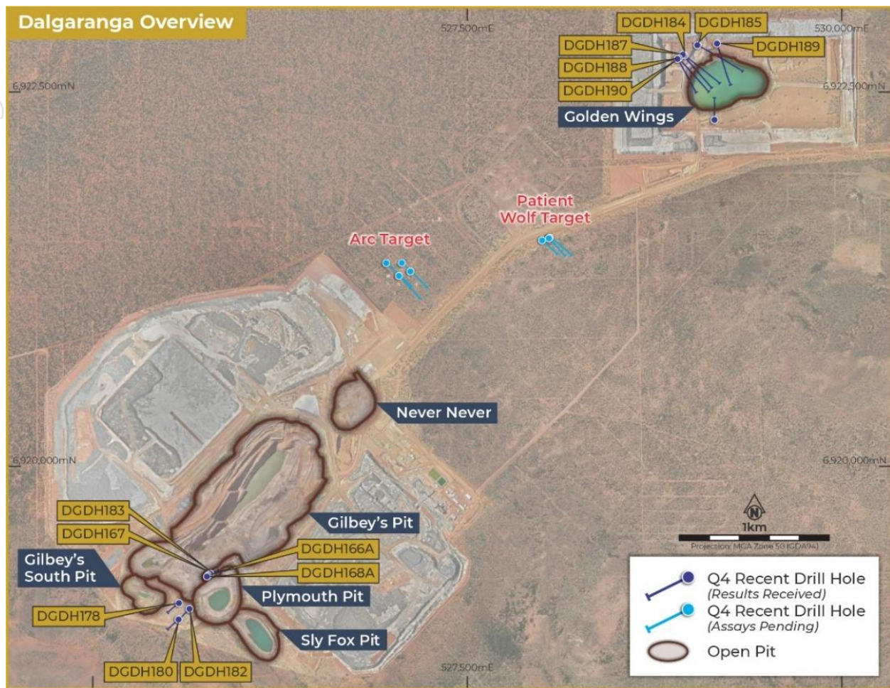
Figure 22: Dalgaranga location map and exploration targets
