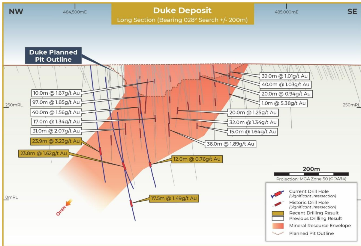
Figure 28: Duke – long section showing recent results
