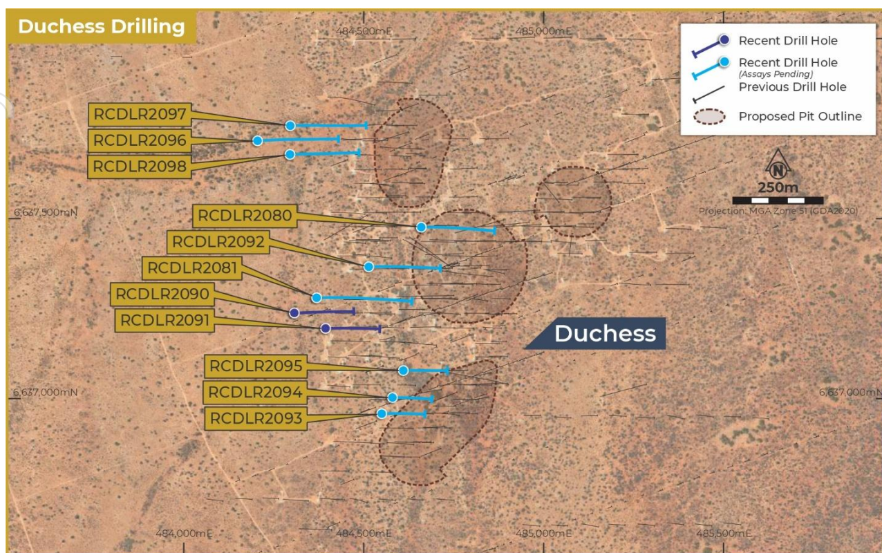
Figure 26: Duchess - drill hole location plan
