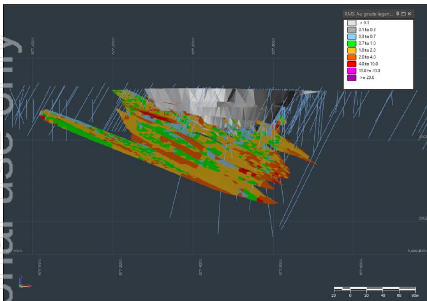
Figure 11: Windbag block model by grade Au. 3-D section facing North. Historic pit in grey.
