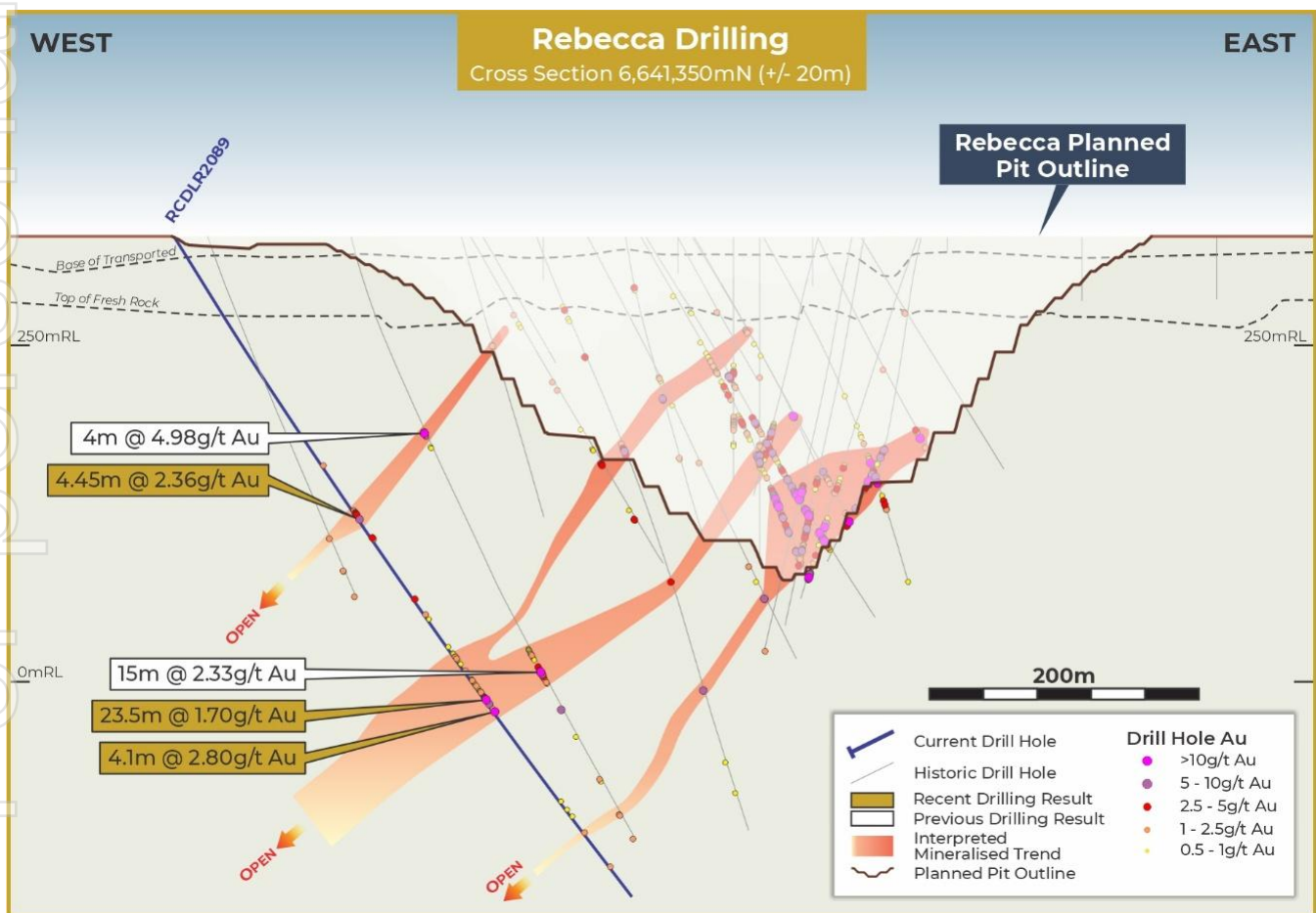
Figure 25: Rebecca - cross section showing recent results
