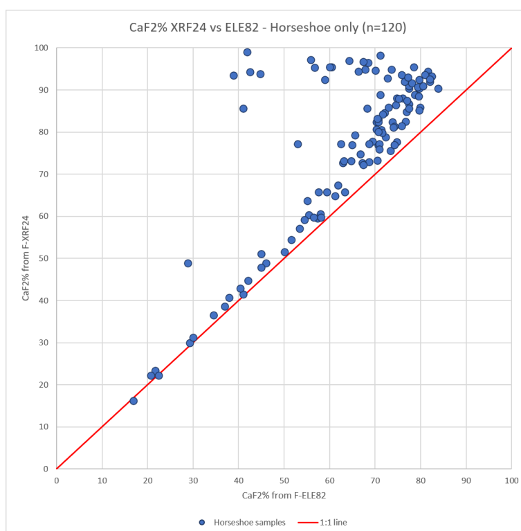
Figure 2 Re-assay program with F-XRF24 versus the original F-ELE82
