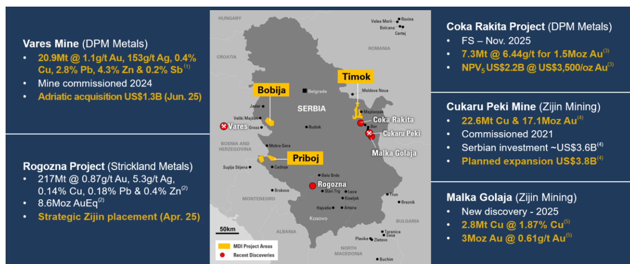
Figure 6: Location of Middle Island projects within world class mineral province.
