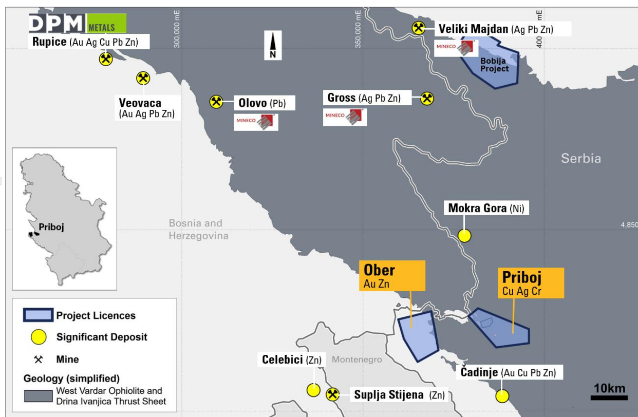
Figure 7: Location of Priboj Project licences and mines / historic workings.
