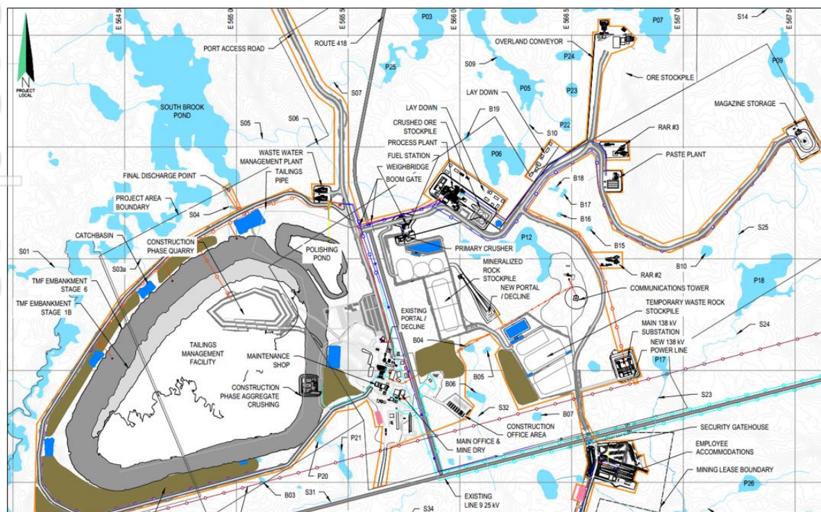
Figure 18: Conceptual site layout for the 4.6Mtpa scenario for development of the Green Bay Ming Mine Project.
