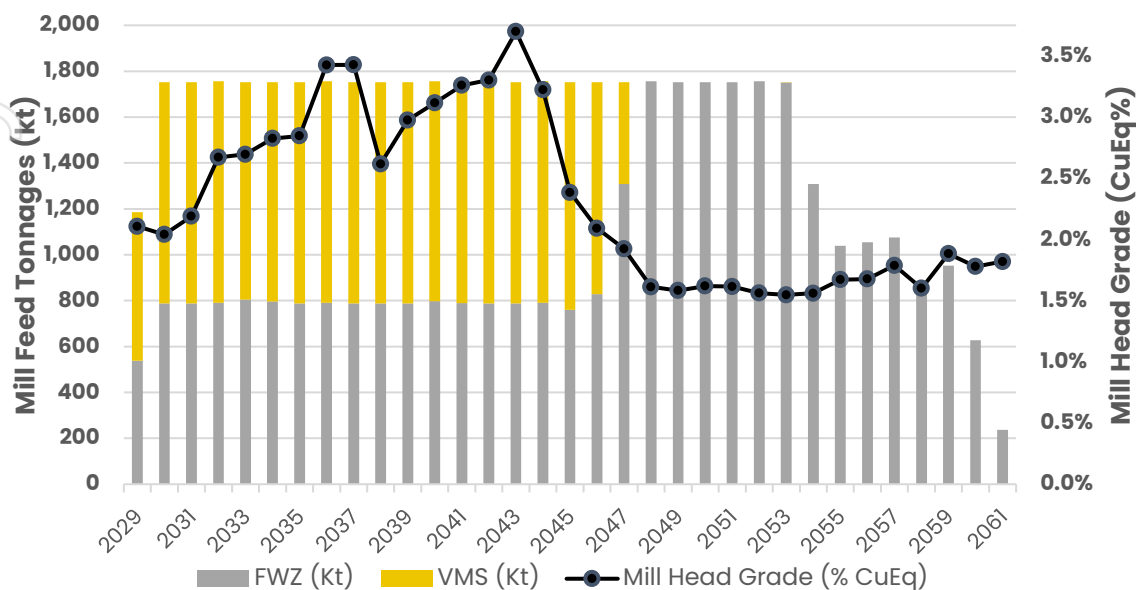
Figure 9: Mined material by mineralisation type for the 1.8Mtpa base case. The VMS mineralisation has been scheduled at the front end of the mine plan to maximise both copper production and minimise the payback period.
