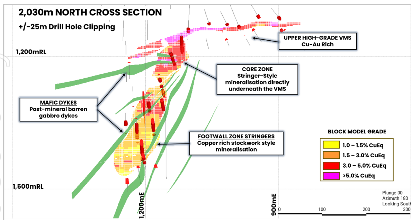
Figure 32: Cross section through the Ming block model showing key geological and mineralisation domains. Red drillholes are grades >0.5% copper. Interpreted post-mineral mafic dykes are shown in green. Clipping +/-25m.
