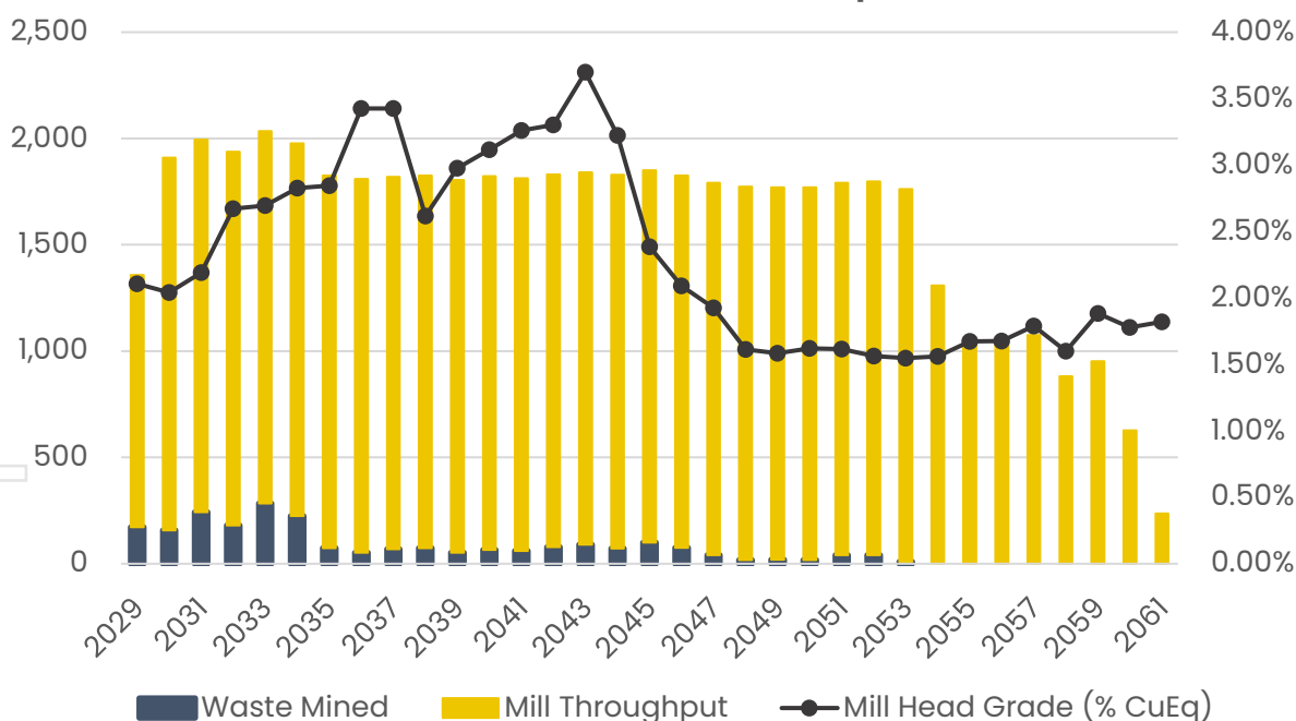
Figure 10: LOM scheduled mine material movement and grade for the 1.8Mtpa base case.
