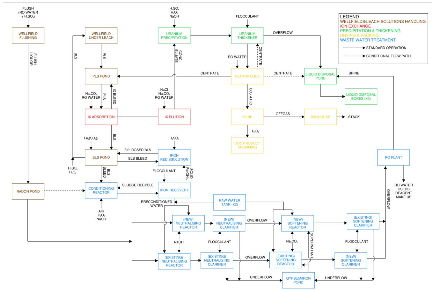
Figure 29: Proposed upgraded Water Treatment Plant Flowsheet
