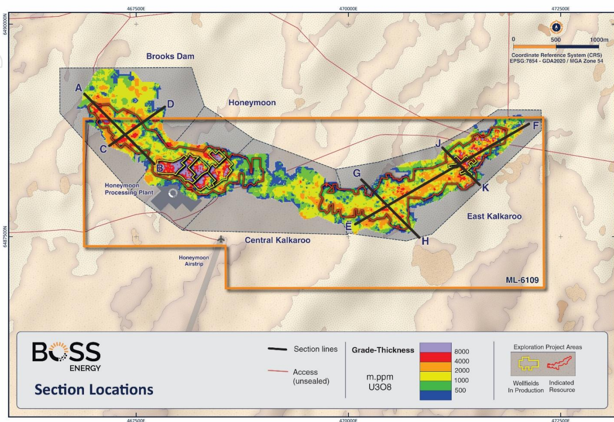
Figure 5: Plan view of the Honeymoon Deposit showing the deposit grade-thickness distribution of Resource blocks at 100 ppm U_3O_8 cut-off with continuous mineralisation over 6 km strike length, and geographical domains. See also the Honeymoon MRE Technical Overview 2026 for additional information.
