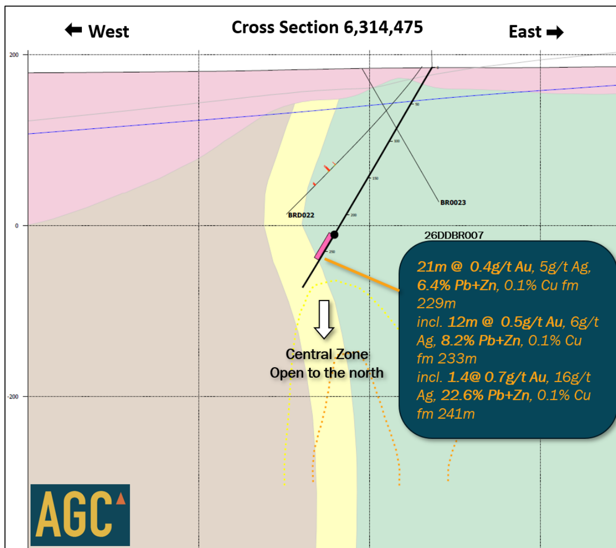
Figure 5: Cross section through 26DDBR007. New results in orange (50m section).
