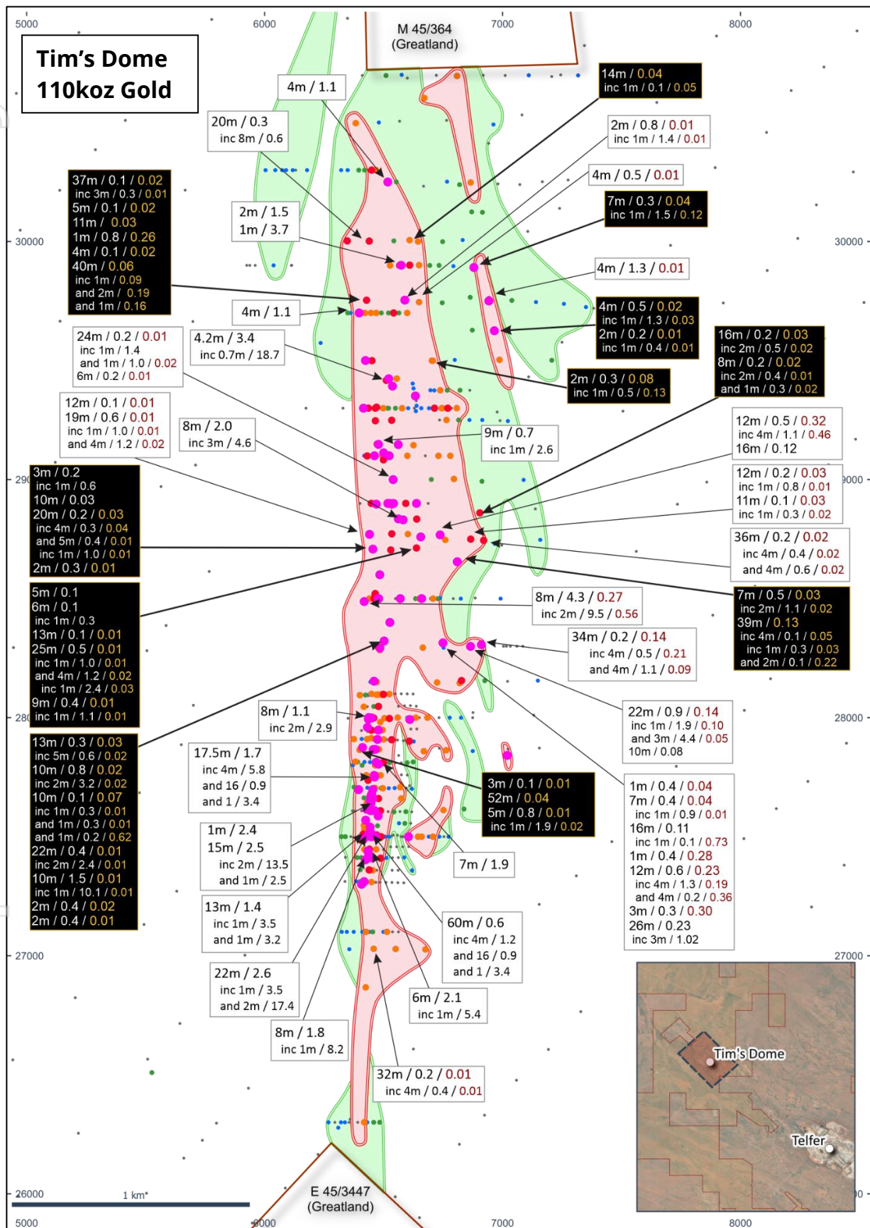
Figure 7: Map showing the Tim's Dome area, including Mineral Resource, contoured maximum down-hole gold drill results and key drill hole gold-copper-lead intercepts (Batch 3 black boxes). NB: Refer to Figures 1, 5 and 6 for location information and Tim's Dome local grid co-ordinates, 1km grid.
