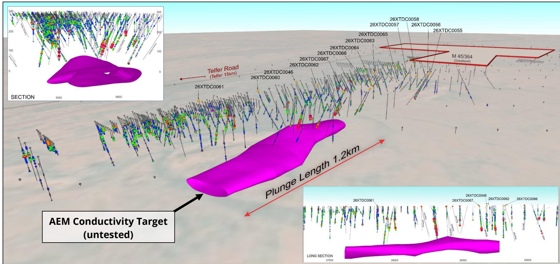
Figure 2: Tim's Dome 3D-perspective (oblique) long-section showing the untested 1.2km long AEM conductivity model (magenta) reef style high-grade gold-copper target: This discrete AEM conductivity anomaly is 270 to 340m below the surface and is also consistent with a Gradient Array Induced Polarisation (GAIP) chargeability anomaly. The Telfer Main Dome mineralisation is preferentially developed along the domal fold axis and eastern fold limb; with bedding parallel high-grade reefs preferentially located where steep cross-cutting ore fluid conduit structures intersect reactive lithologies/contacts. This AEM conductivity anomaly overlaps the Tim's Dome fold axis and is predominantly located within the eastern fold limb of the dome. Refer also to cross-sections Figures 3 and 4 and conceptual structural model 3D-perspective long-section Figure 8 and cross-section Figure 9, and Figure 7 for location information. View bearings for 3D-perspective image -35° to 270° and inset cross-section 0° to 320° and inset long-section 0° to 225°. NB: Tim's Dome Local Grid.
