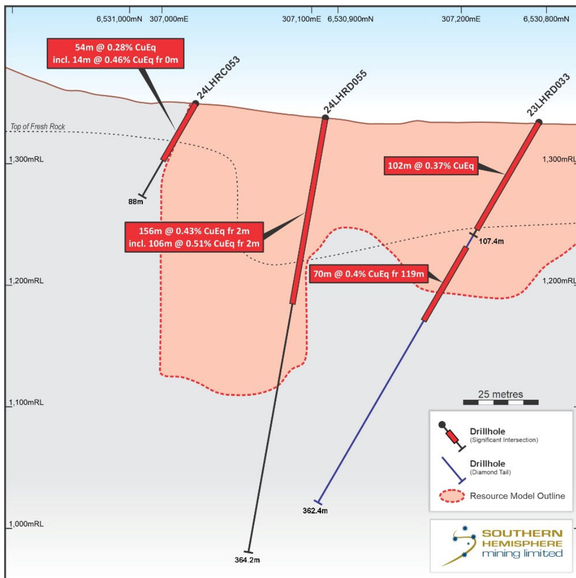
Figure 3. Section with 23LHRD033
