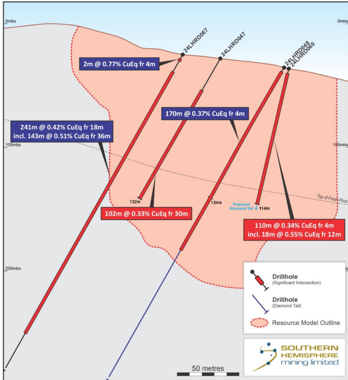
Figure 2. Section with 24LHRD048
