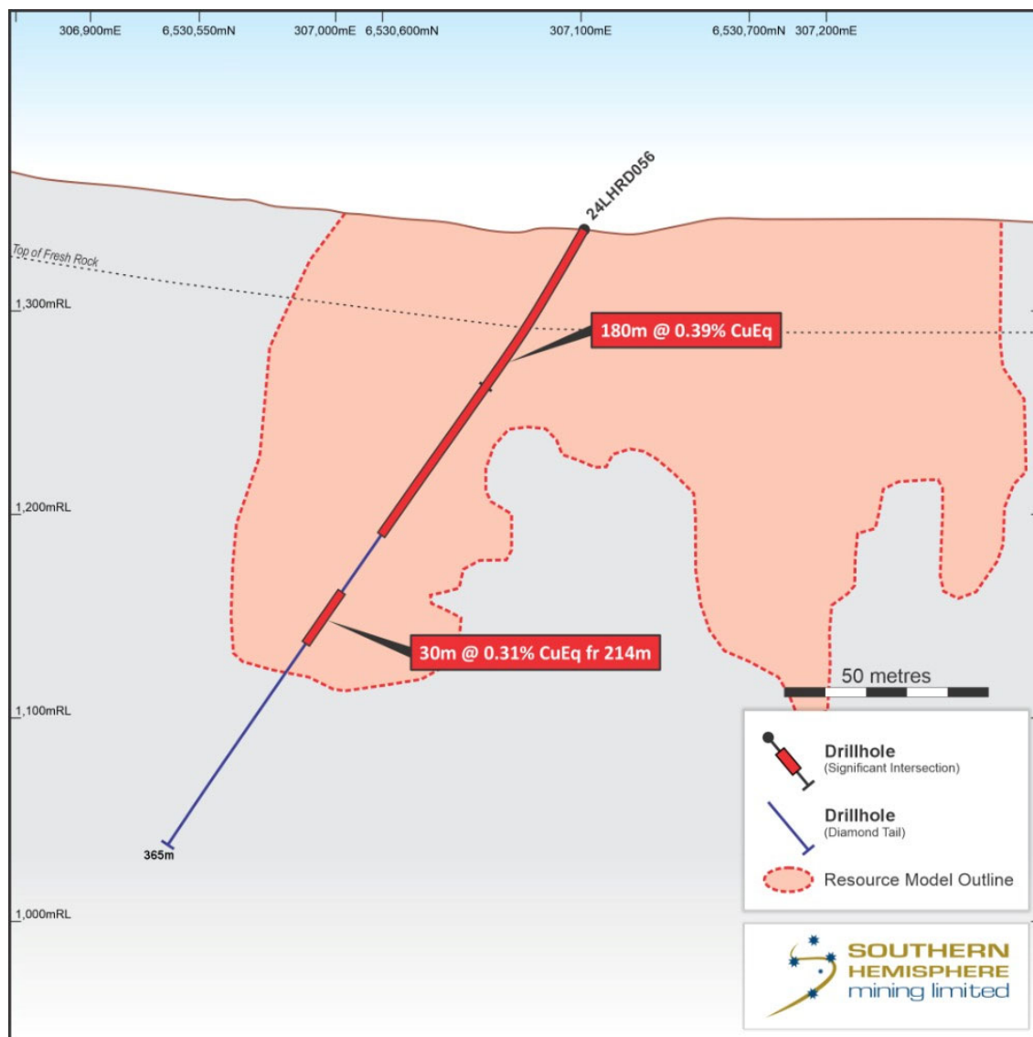
Figure 1. Section with 24LHRD056
