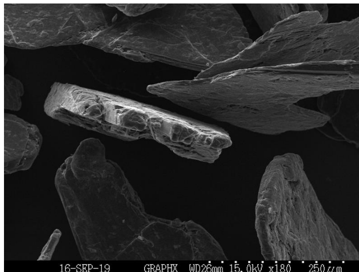
Figure 1. Chilalo +80 mesh concentrate before intercalation (GN190904003). Original AETC SEM image, CC1953-001
