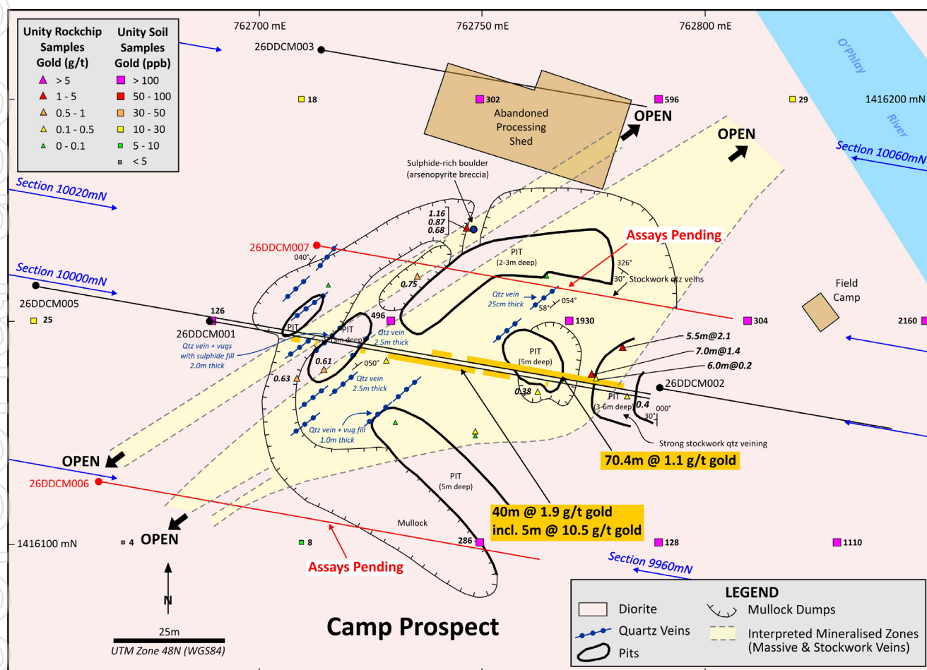
Figure 3: Location of the broad gold mineralised zone discovered in the eastern portion of the Camp Prospect showing drill holes, historical mine workings, soil sample gold results & rockchip sample gold results on geological mapping.
