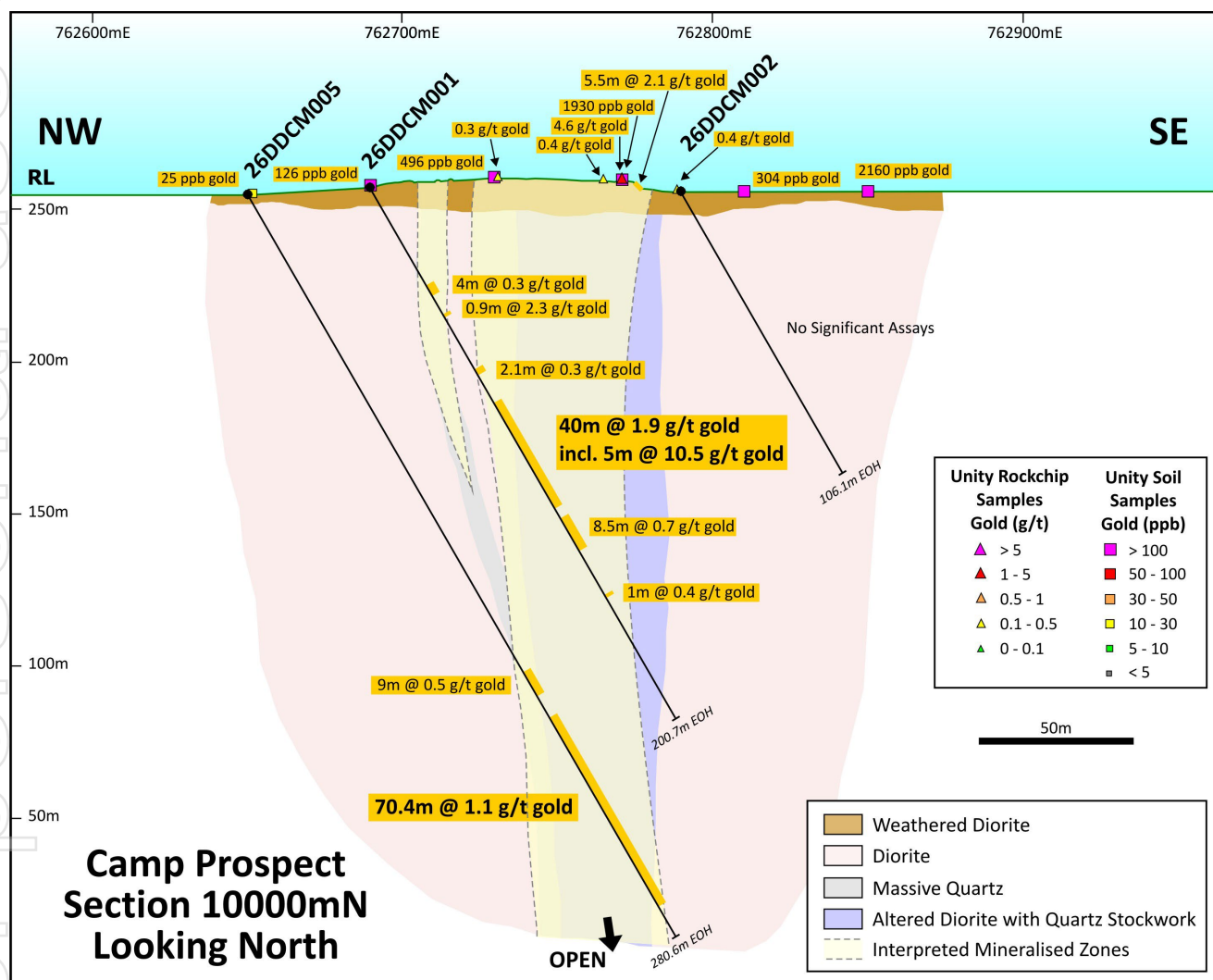
Figure 1: Drilling Cross Section 10,000mN at Camp Prospect with gold intersections and a geological interpretation.
