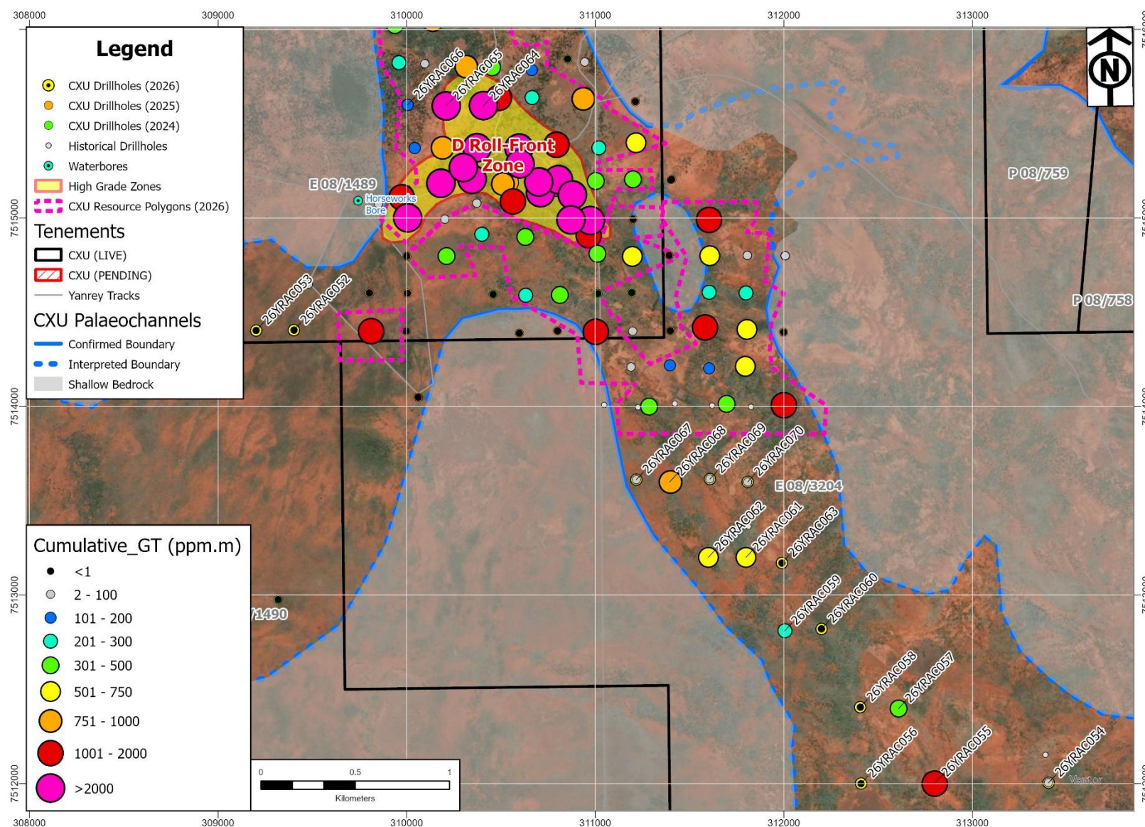
Figure 7. Manyingee South Cumulative GT (ppm*m) map.
