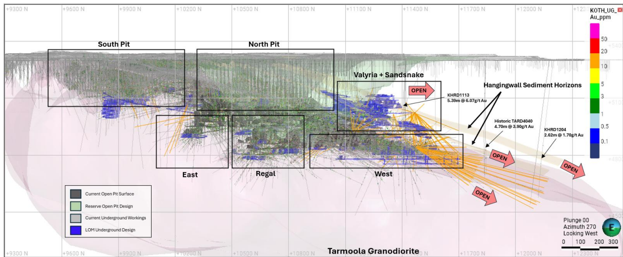
Figure 3: KoTH Long Section showing planned FY27 drilling
