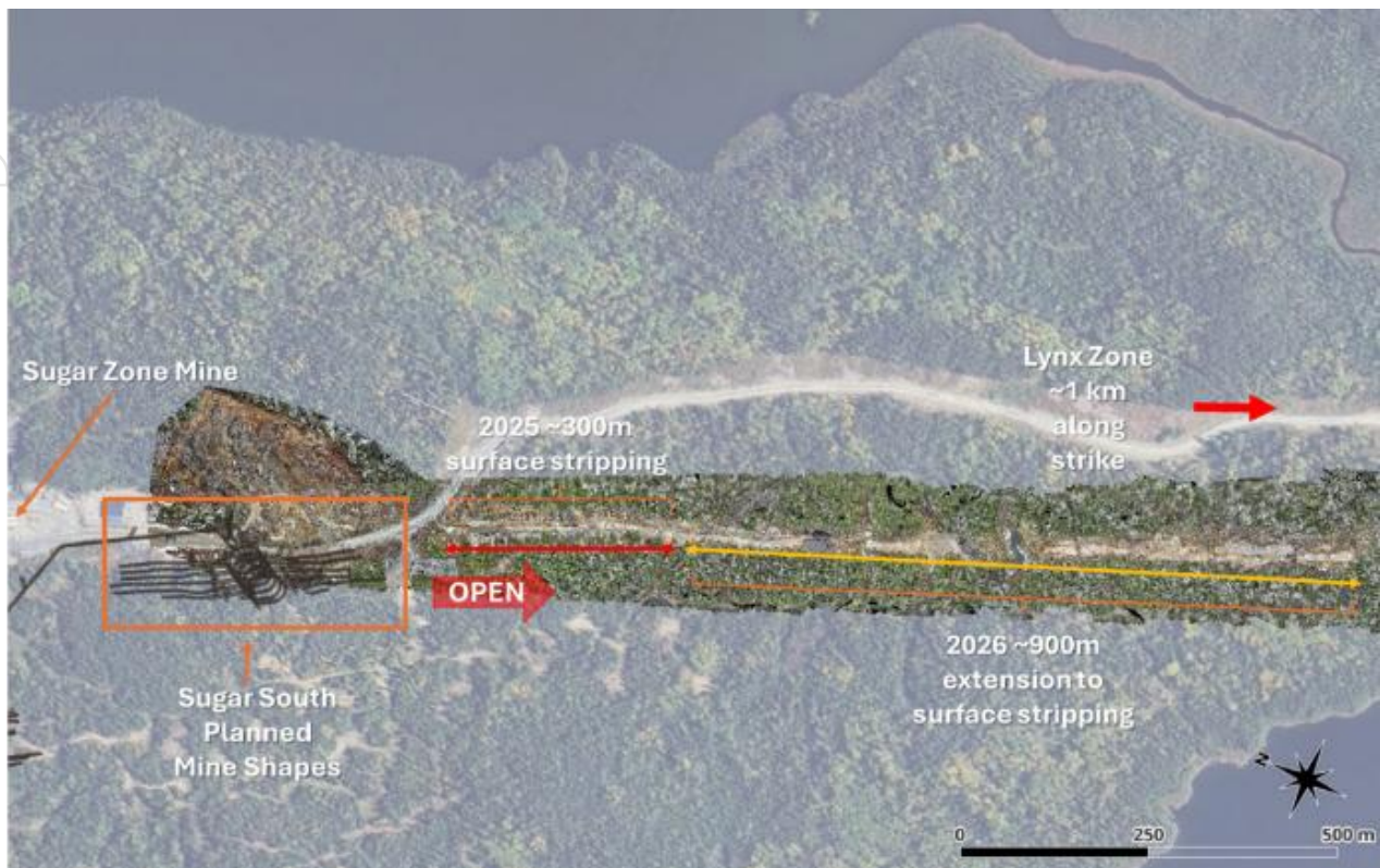
Figure 12: Surface stripping along the southern Sugar Zone mine corridor
