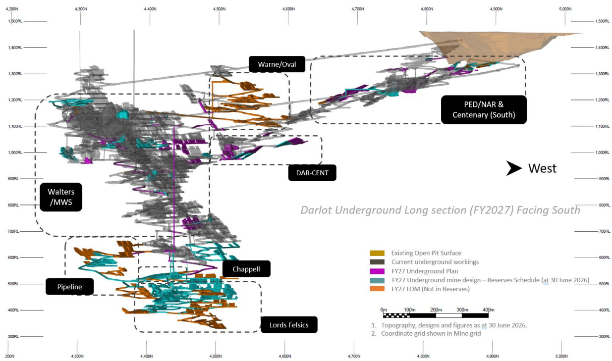
Figure 4: Darlot long section highlighting Ore Reserve relative to life of mine designs outside of Ore Reserve
