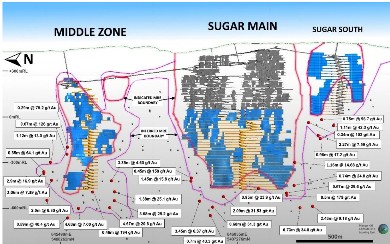
Figure 11: Sugar Zone Ore Reserve design relative to Indicated Mineral Resource boundary and exploration results beyond the Indicated Mineral Resource boundary (Drill results previously released 2 )
