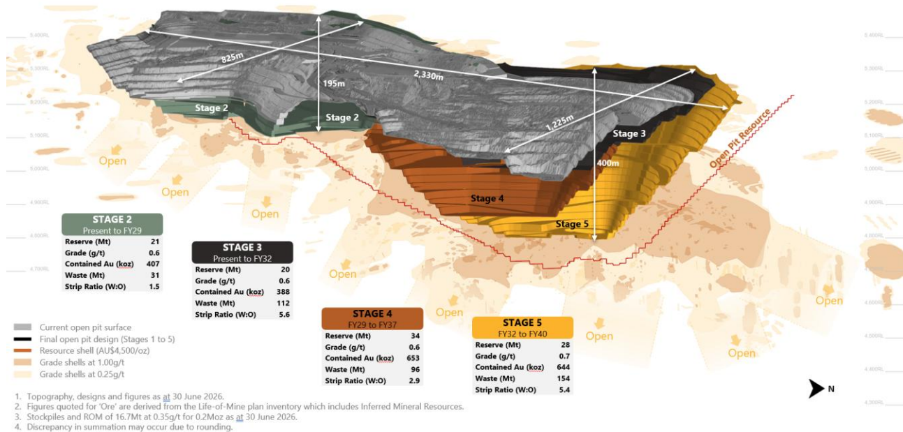
Figure 1: King of the Hills open pit Ore Reserve pit shell and open pit development stages
