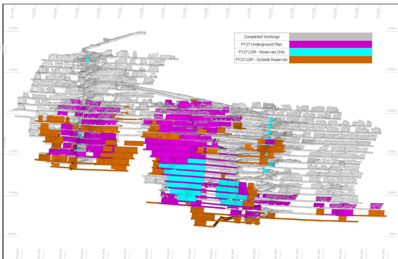
Figure 10: Rothsay FY27 mine schedule (purple) v Ore Reserves LOM (light blue)
