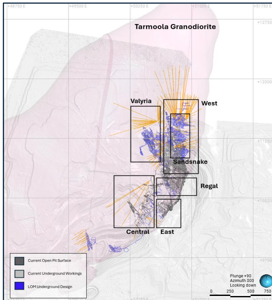
Figure 2: Plan view of KoTH underground highlighting mining areas and FY27 planned exploration drilling
