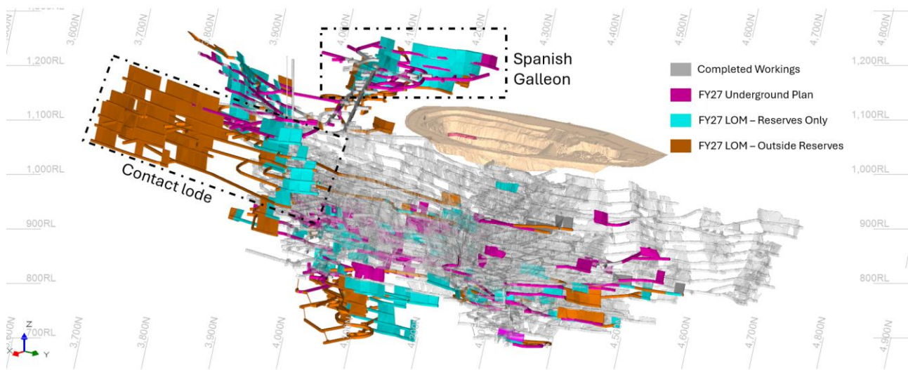
Figure 8: Deflector FY27 mine schedule v Ore Reserves LOM including Contact Lode shapes outside of Ore Reserves demonstrating opportunity for conversion and extension
