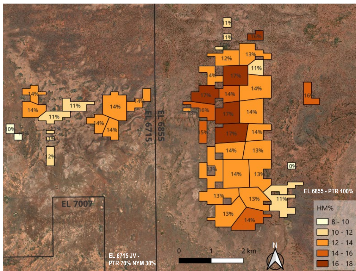
Figure 1: Example RF50 Pit Shell and Mining Blocks, labelled by HM% in scheduled plant feed.
