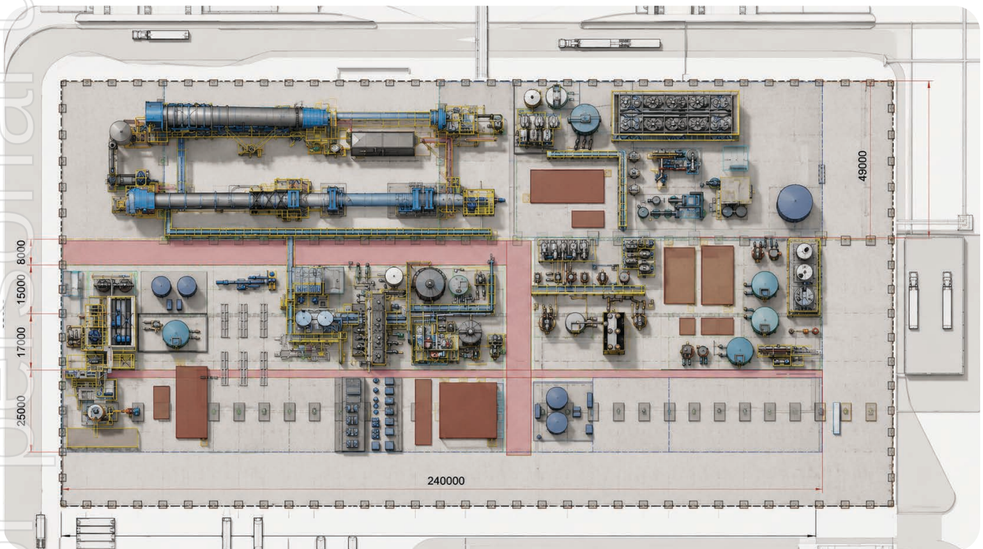
Figure 18: Lithium Universe Proposed Brownsville Refinery Plant Internal Layout
